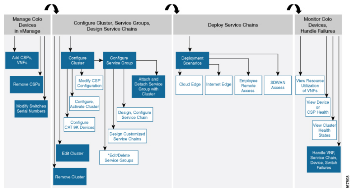
Figure 32: Day-N Workflow
