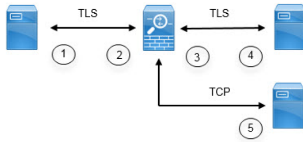
Figure 48: Diameter TLS Inspection
