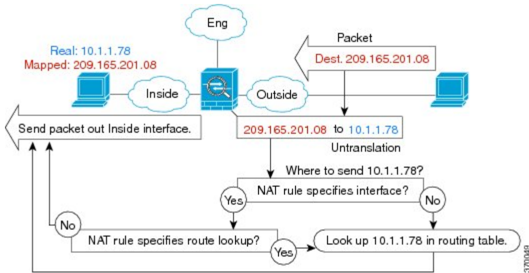
Figure 38: Routed Mode Egress Interface Selection with NAT
