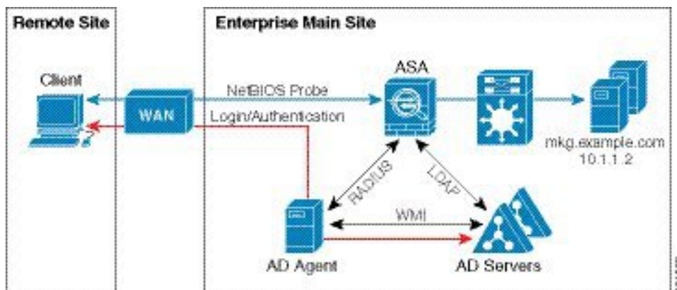
Figure 7: WAN-based Deployment
