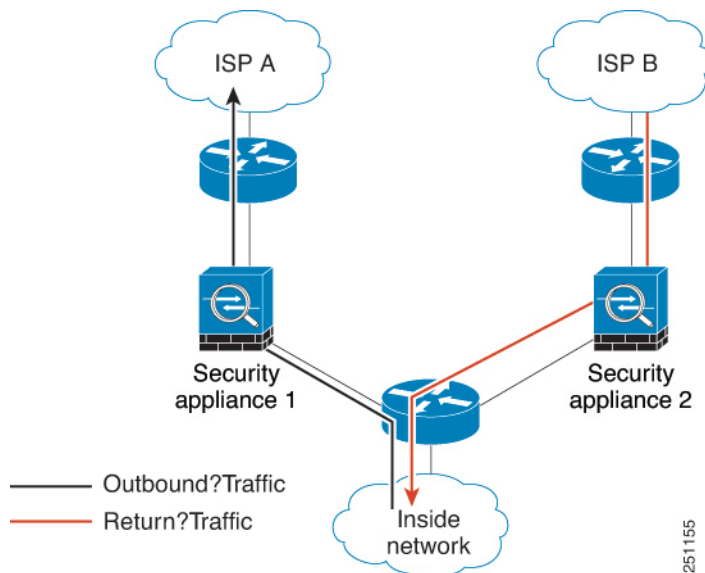
Figure 49: Asymmetric Routing
