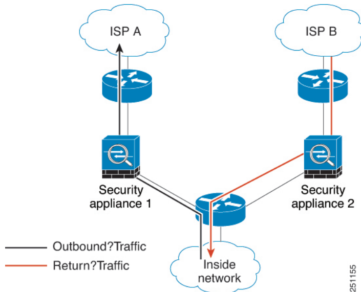
Figure 53: Asymmetric Routing
