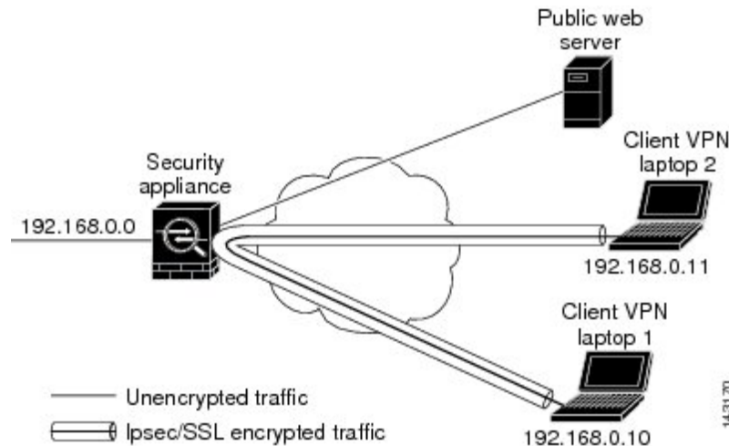
Figure 3: VPN Client Using Intra-Interface Feature for Hairpinning
