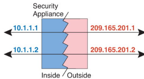
Figure 21: Static NAT
