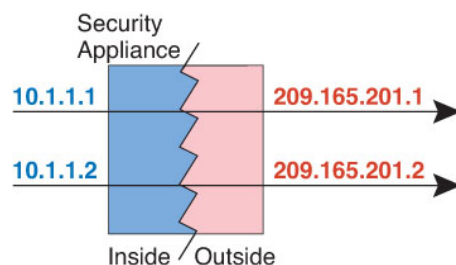
Figure 18: Dynamic NAT
