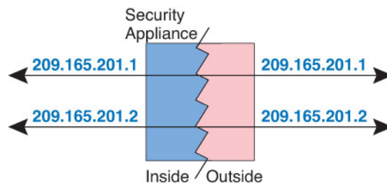
Figure 27: Identity NAT
