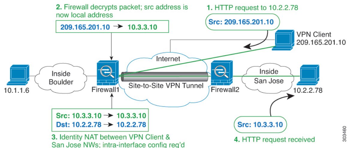
Figure 42: VPN Client Access to Site-to-Site VPN
