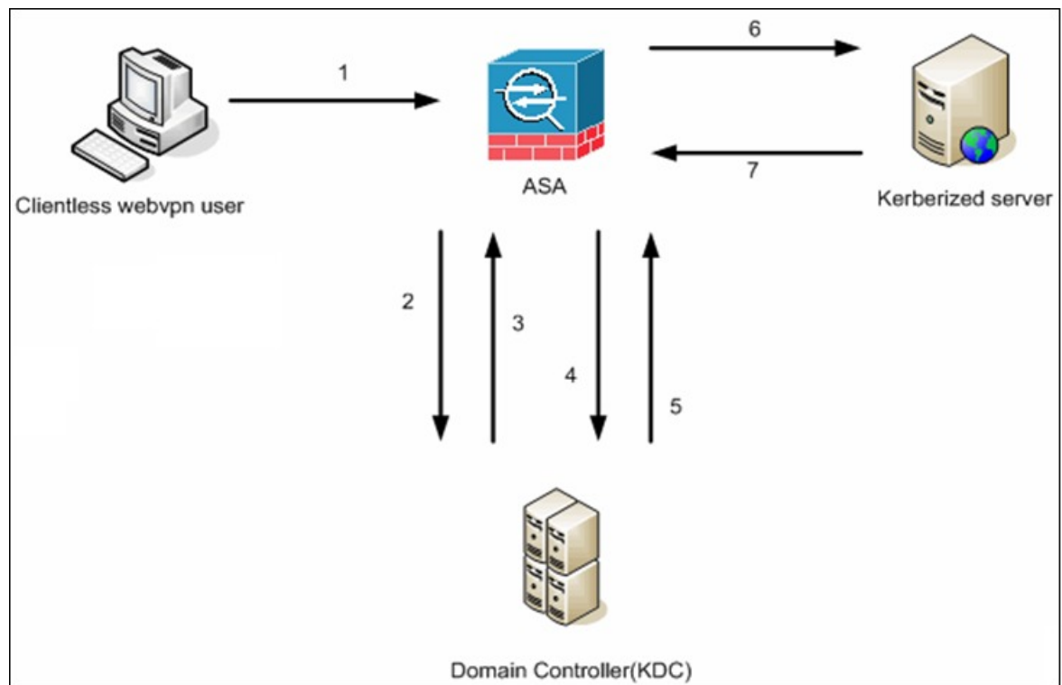
Figure 10: KCD Process
