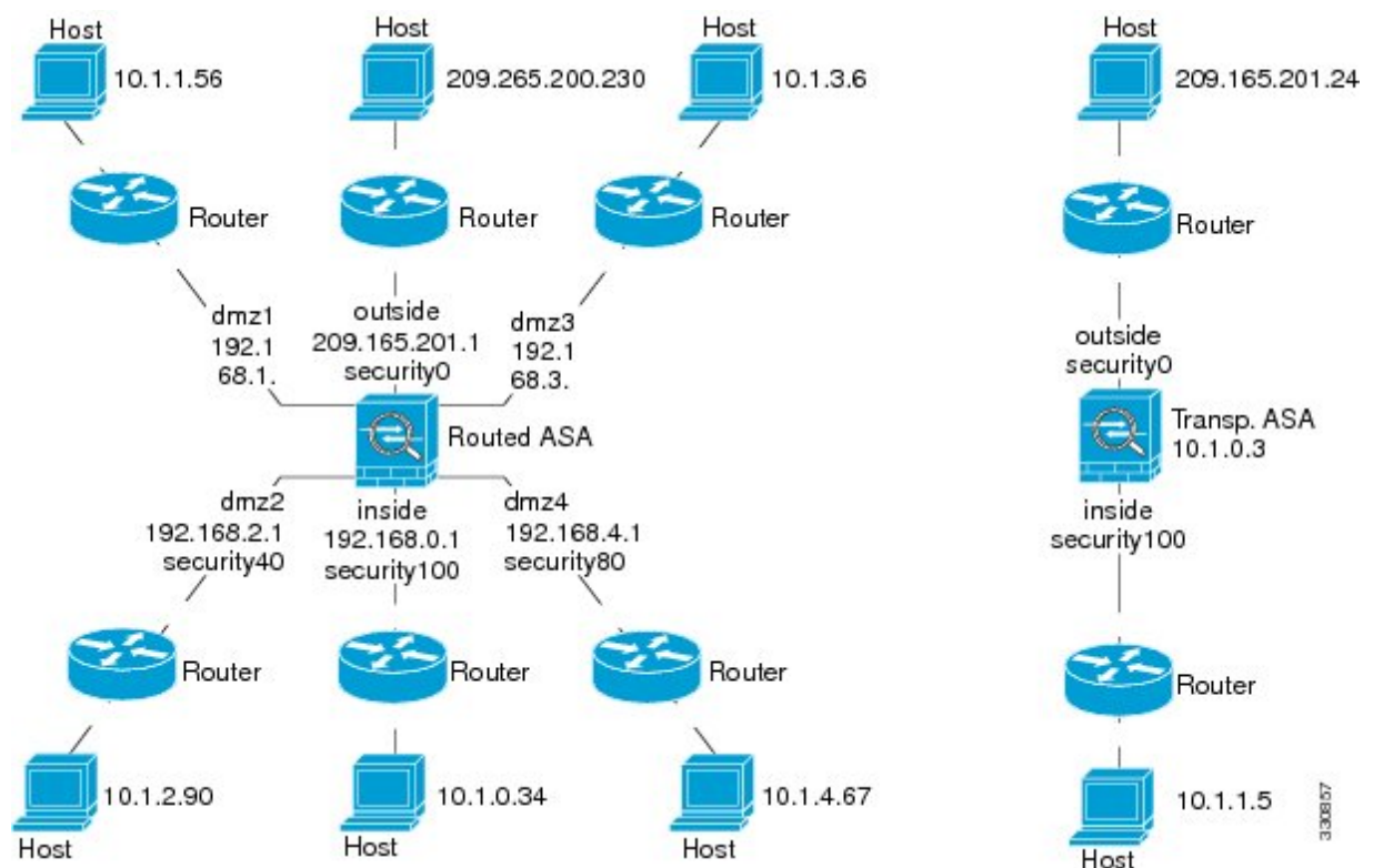
Figure 1: Network Diagram with Interfaces, Routers, and Hosts
