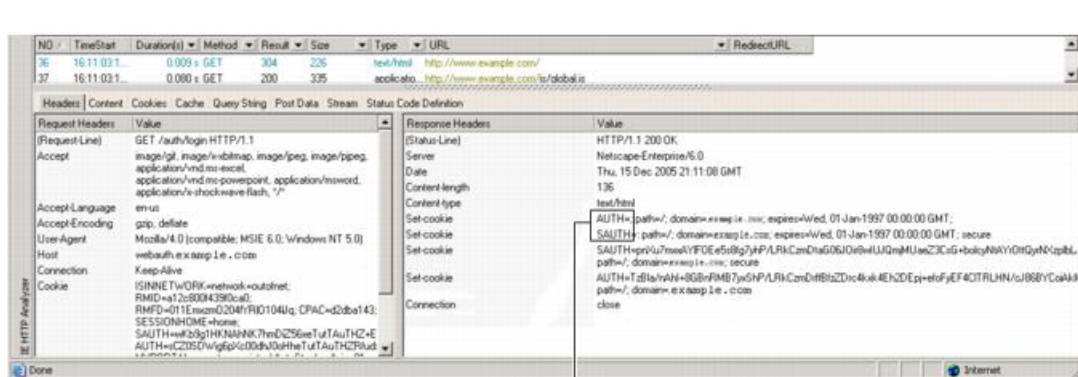
Figure 12: Authorization Cookies in Sample HTTP Analyzer Output
