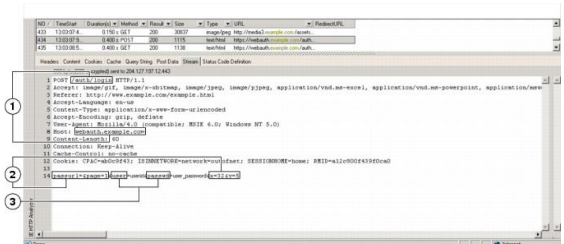
Figure 11: Action-uri, hidden, username and password parameters
