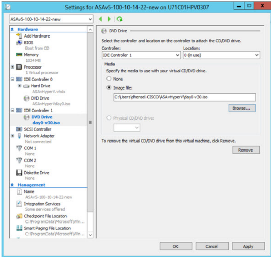
Figure 38: Hyper-V Manager
