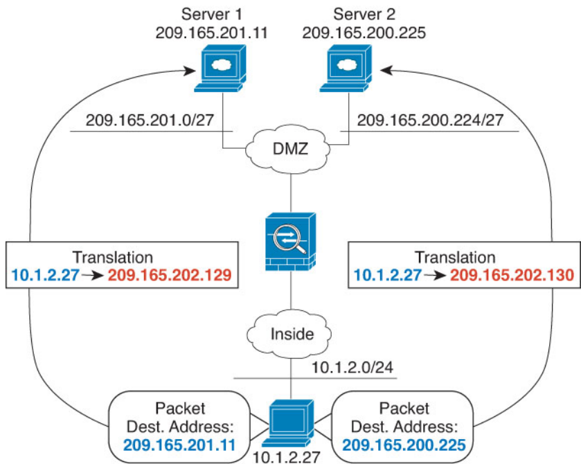
Figure 32: Twice NAT with Different Destination Addresses
