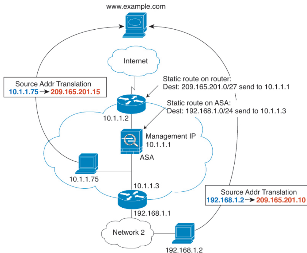
Figure 35: NAT Example: Transparent Mode
