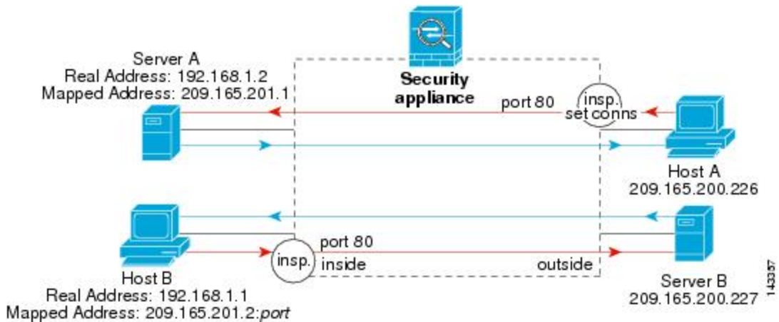
Figure 49: HTTP Inspection and Connection Limits to Specific Servers
