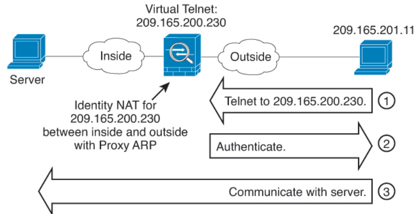
Figure 37: Proxy ARP and Virtual Telnet
