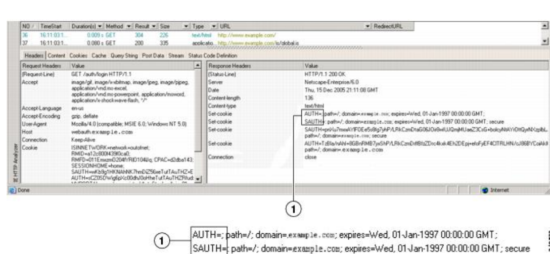
Figure 12: Authorization Cookies in Sample HTTP Analyzer Output
