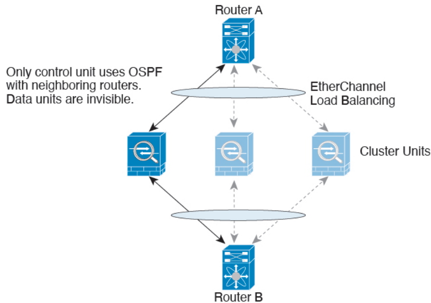
Figure 48: Dynamic Routing
