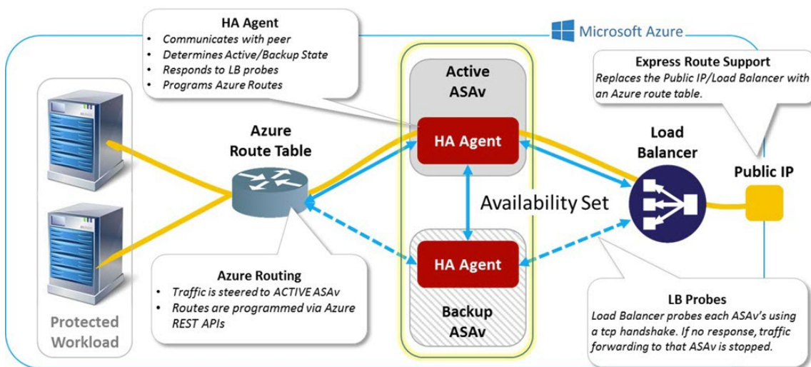
Figure 45: ASAv HA Deployment in Azure
