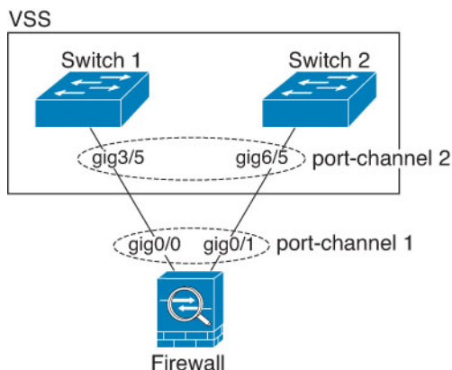
Figure 52: Connecting to a VSS/vPC
