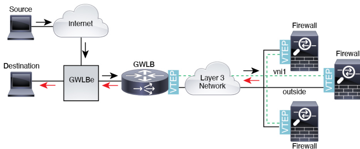
Figure 54: Geneve Single-Arm Proxy
