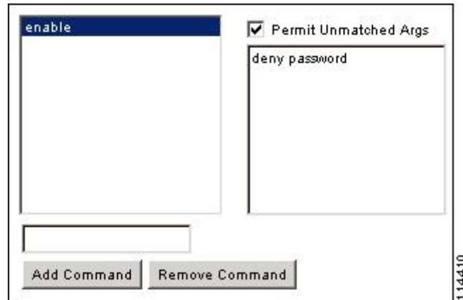
Figure 67: Disallowing Arguments
