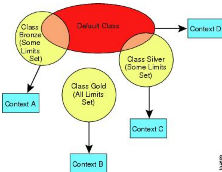
Figure 36: Resource Classes
