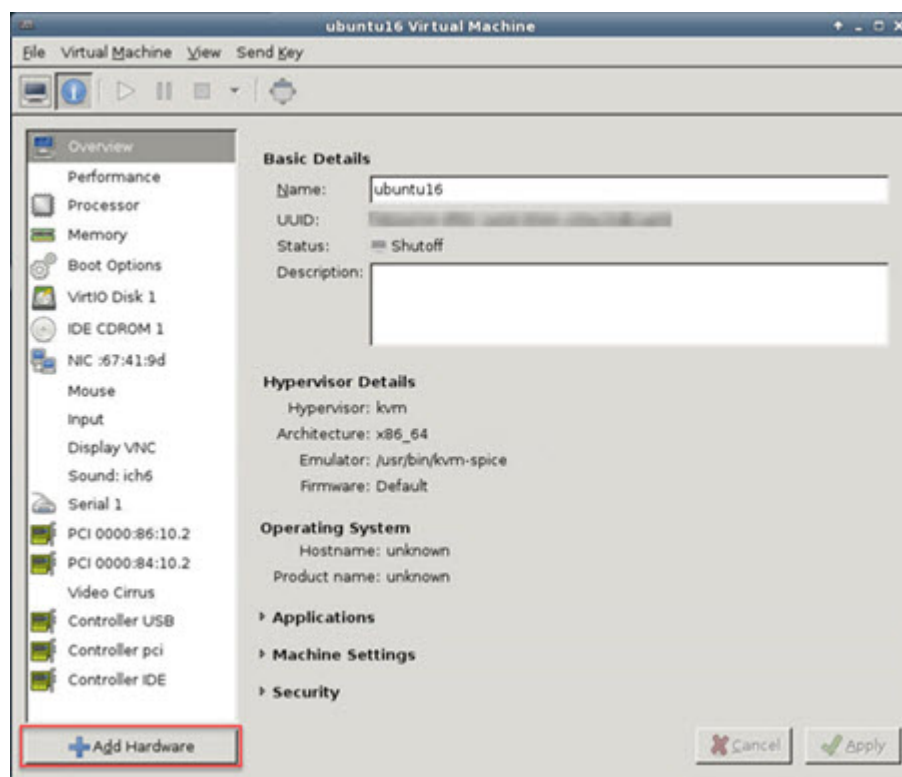
Figure 6: Add Hardware
