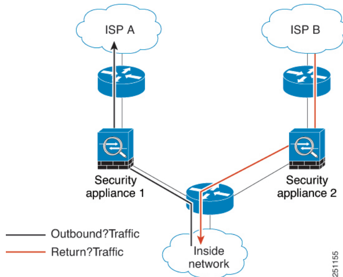
Figure 44: Asymmetric Routing
