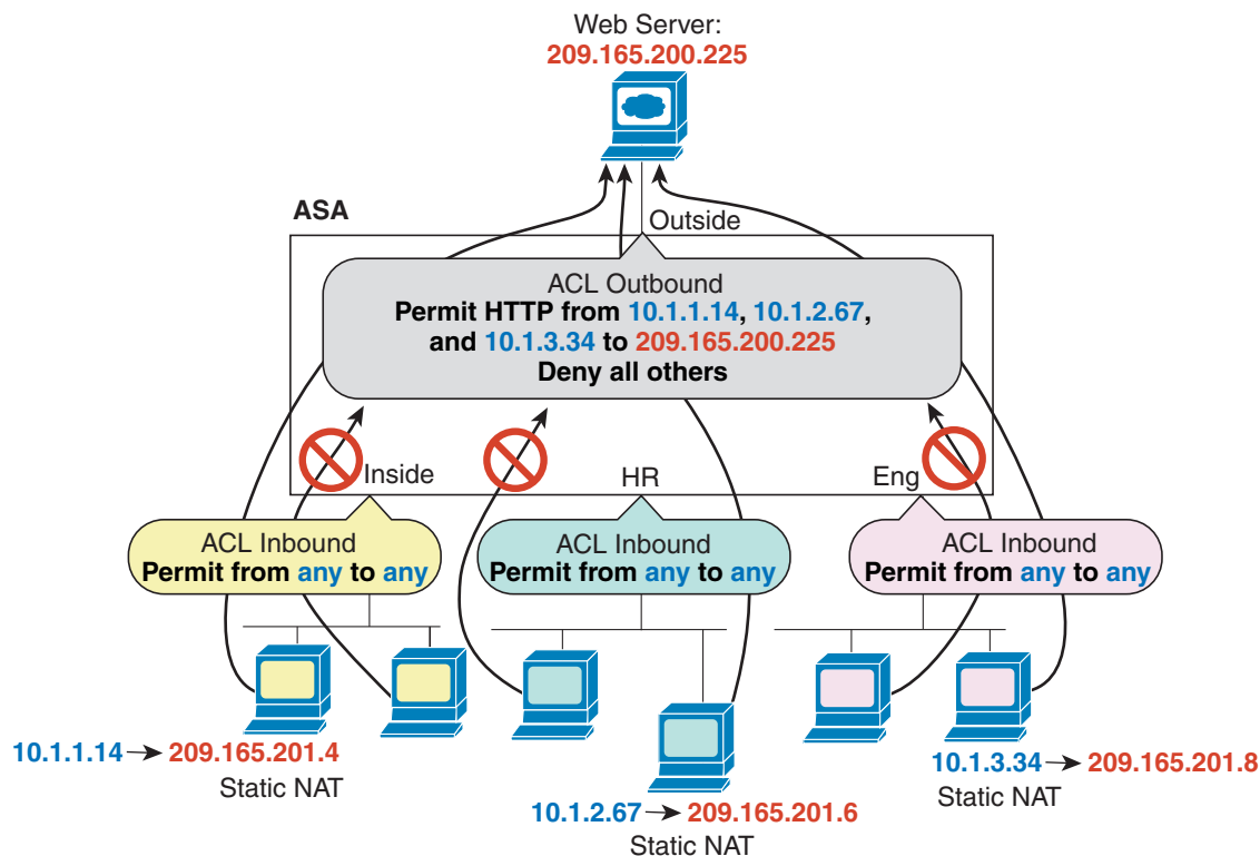
Figure 3-1 Outbound ACL
