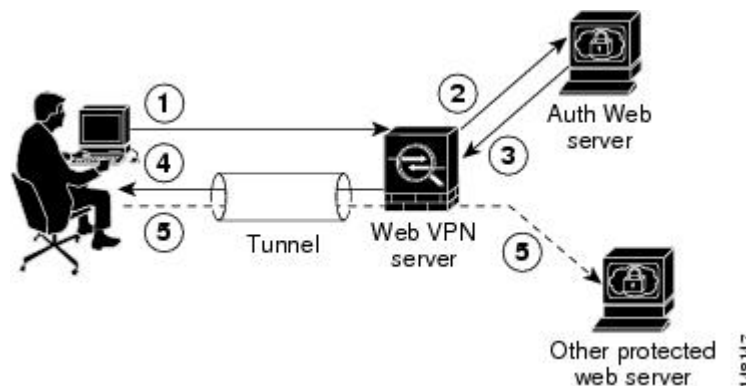
Figure 9: SSO Authentication Using HTTP Forms
