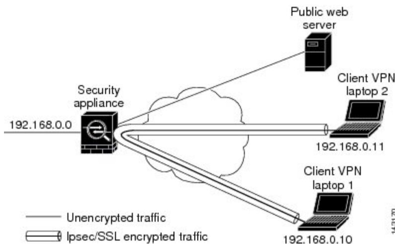
Figure 3: VPN Client Using Intra-Interface Feature for Hairpinning
