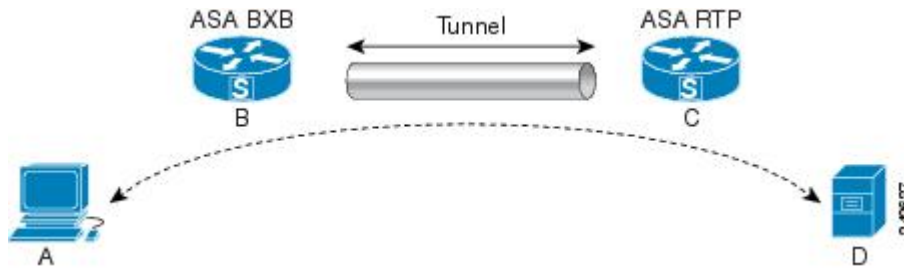
Figure 4: Network Scenario
