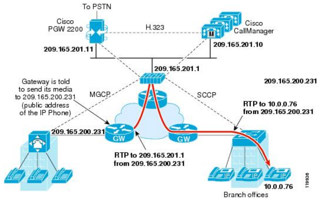
Figure 45: Using NAT with MGCP
