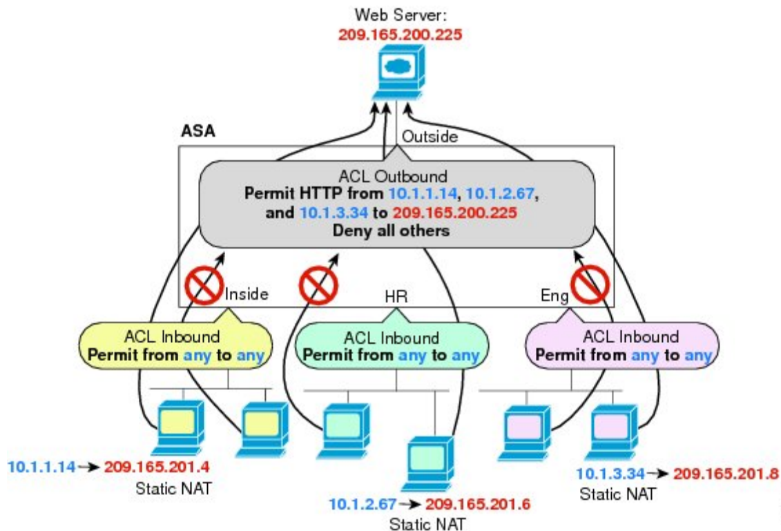
Figure 2: Outbound ACL
