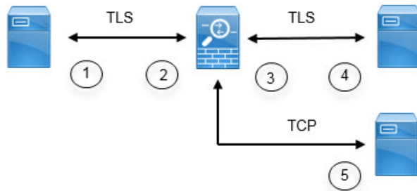
Figure 47: Diameter TLS Inspection
