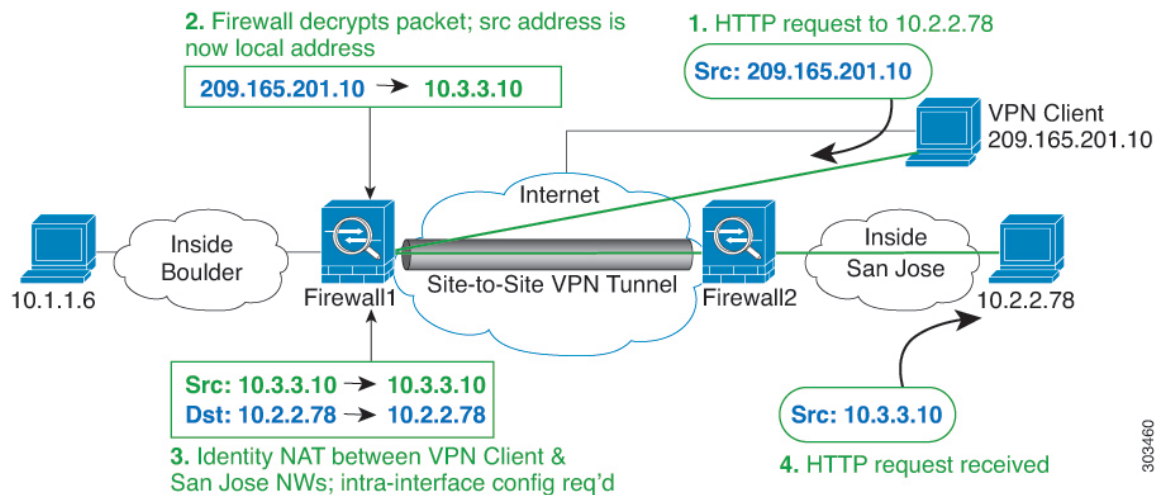
Figure 41: VPN Client Access to Site-to-Site VPN
