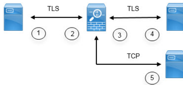
Figure 51: Diameter TLS Inspection
