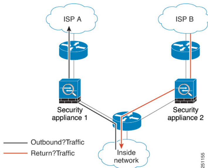
Figure 52: Asymmetric Routing
