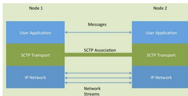
Figure 50: Relationship Between SCTP Association and Streams
