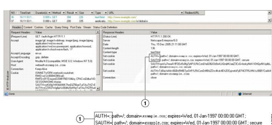
Figure 11: Authorization Cookies in Sample HTTP Analyzer Output
