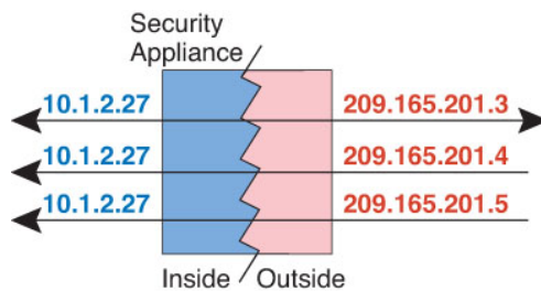
Figure 23: One-to-Many Static NAT
