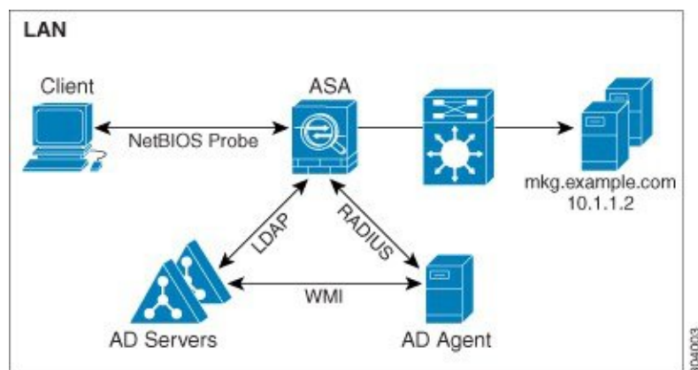
Figure 6: LAN-based Deployment
