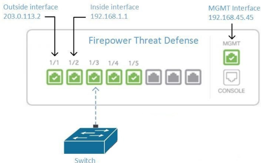
Figure 6: Interface Addresses
