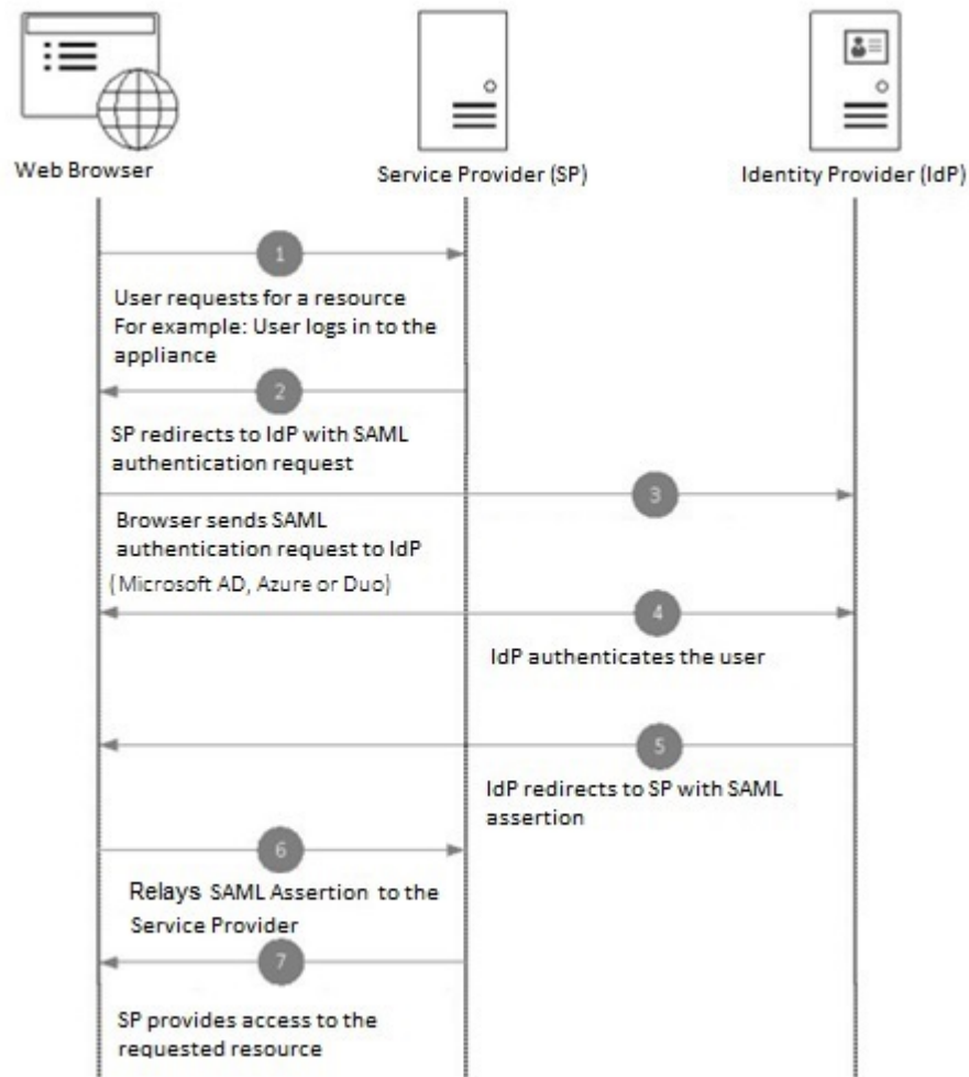
Figure 77: SAML Workflow
