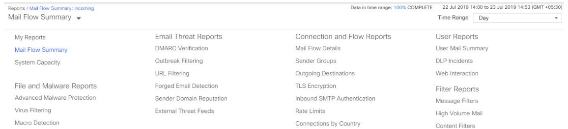
Figure 71: Reports Drop-down
