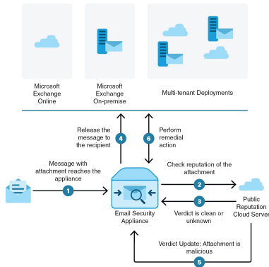
Figure 36: Mailbox Auto Remediation Workflow
