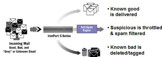
Figure 14: Sender Reputation Filtering Example
