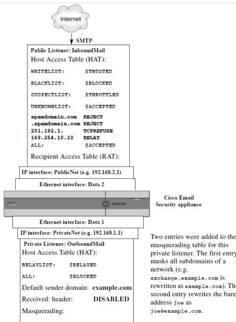
Figure 49: Masquerading Defined for a Private Listener
