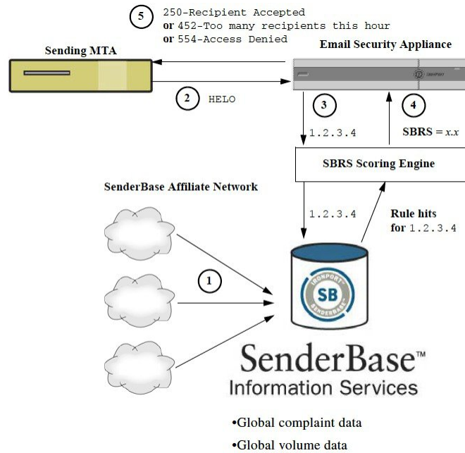
Figure 13: The SenderBase Reputation Service
