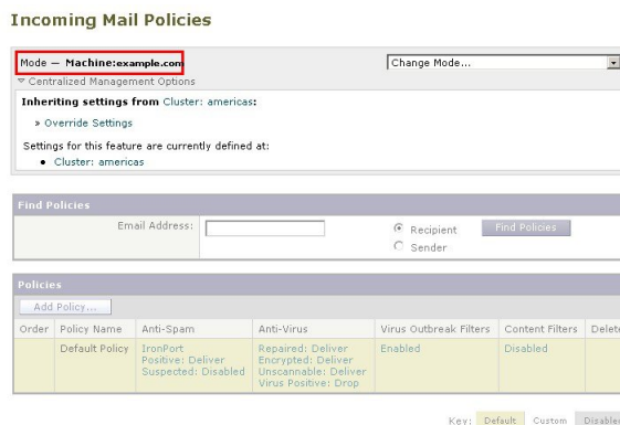
Figure 81: Centralized Management Feature in the GUI: No Settings Defined
