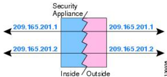
Figure 12: Identity NAT
