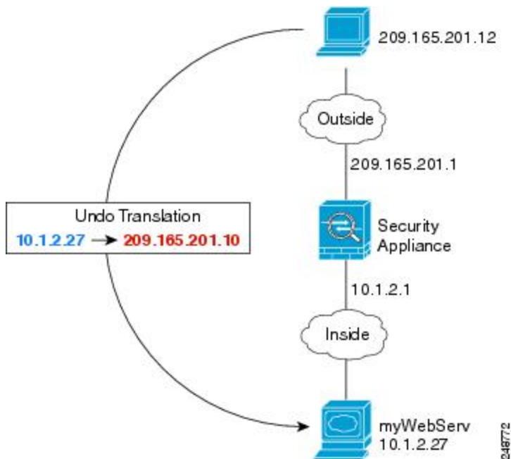
Figure 13: Static NAT for an Inside Web Server
