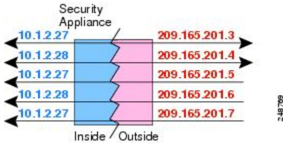
Figure 10: Few-to-Many Static NAT
