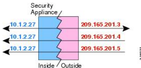
Figure 8: One-to-Many Static NAT
