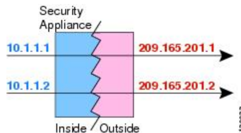
Figure 3: Dynamic NAT
