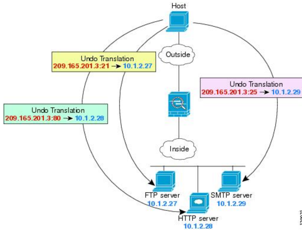
Figure 14: Static NAT-with-Port-Translation
