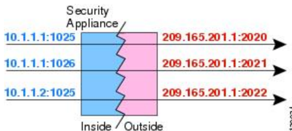
Figure 5: Dynamic PAT
