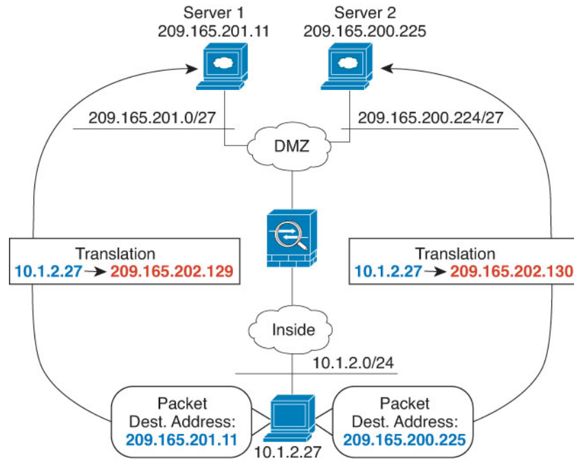
Figure 15: Manual NAT with Different Destination Addresses
