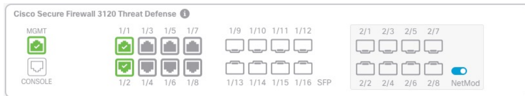
Figure 29: Disable Network Module
