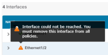
Figure 26: Removed Interfaces
