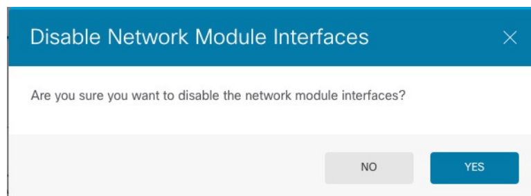
Figure 23: Confirm Disable
