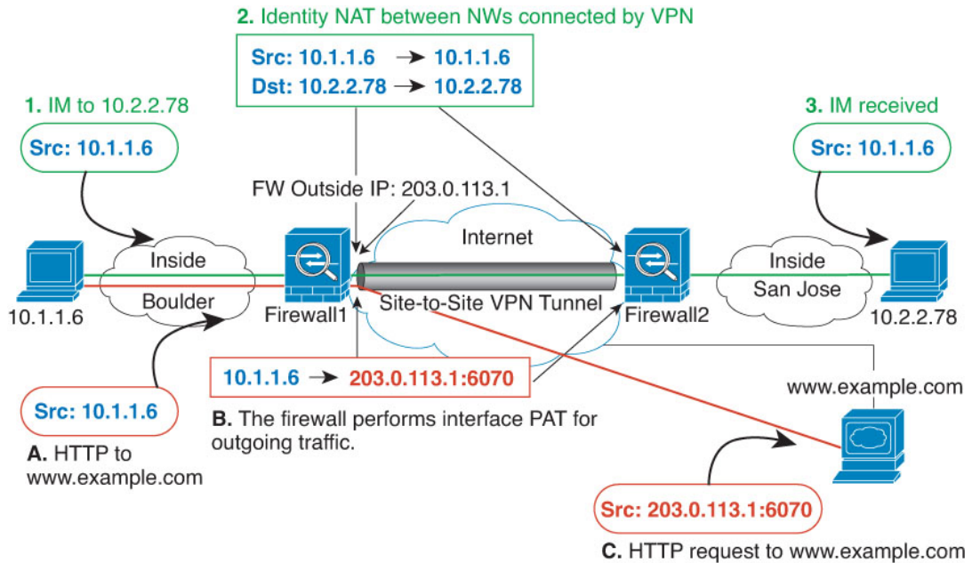
Figure 49: Interface PAT and Identity NAT for Site-to-Site VPN
