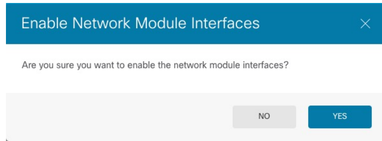
Figure 28: Confirm Enable
