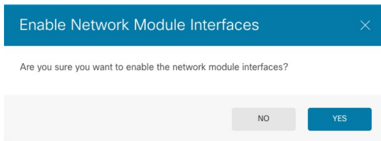
Figure 21: Confirm Enable
