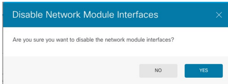
Figure 30: Confirm Disable
