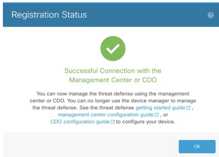
Figure 51: Successful Connection
