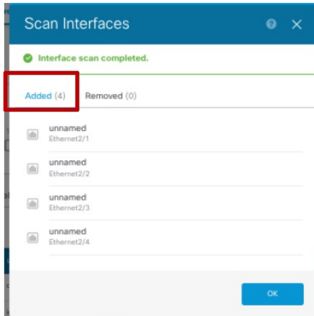
Figure 25: Scan Interfaces
