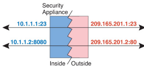
Figure 39: Typical Static NAT with Port Translation Scenario
