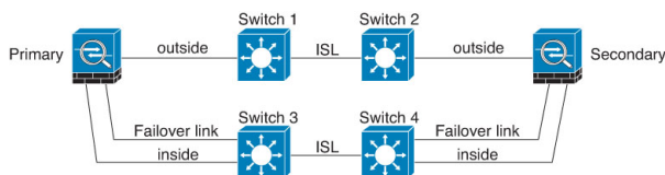
Figure 11: Connecting with a Secure Switch
