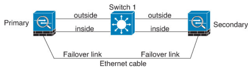
Figure 10: Connecting with a Cable
