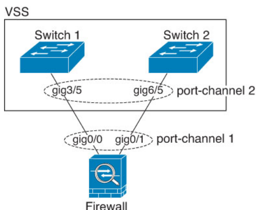
Figure 12: Connecting to a VSS/vPC
