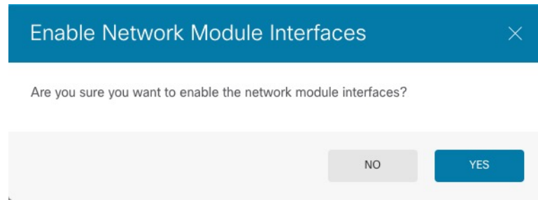
Figure 28: Confirm Enable
