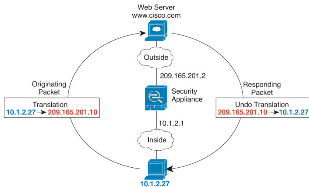
Figure 35: NAT Example: Routed Mode
