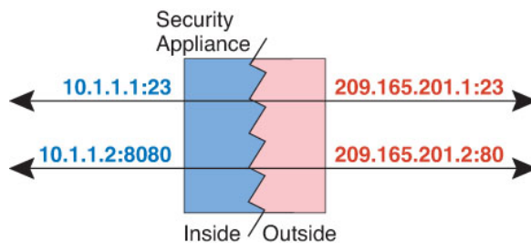
Figure 41: Typical Static NAT with Port Translation Scenario
