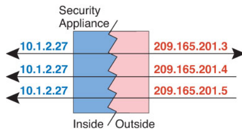
Figure 42: One-to-Many Static NAT
