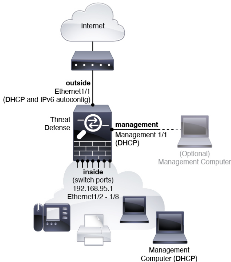
Figure 59: Suggested Network Deployment
