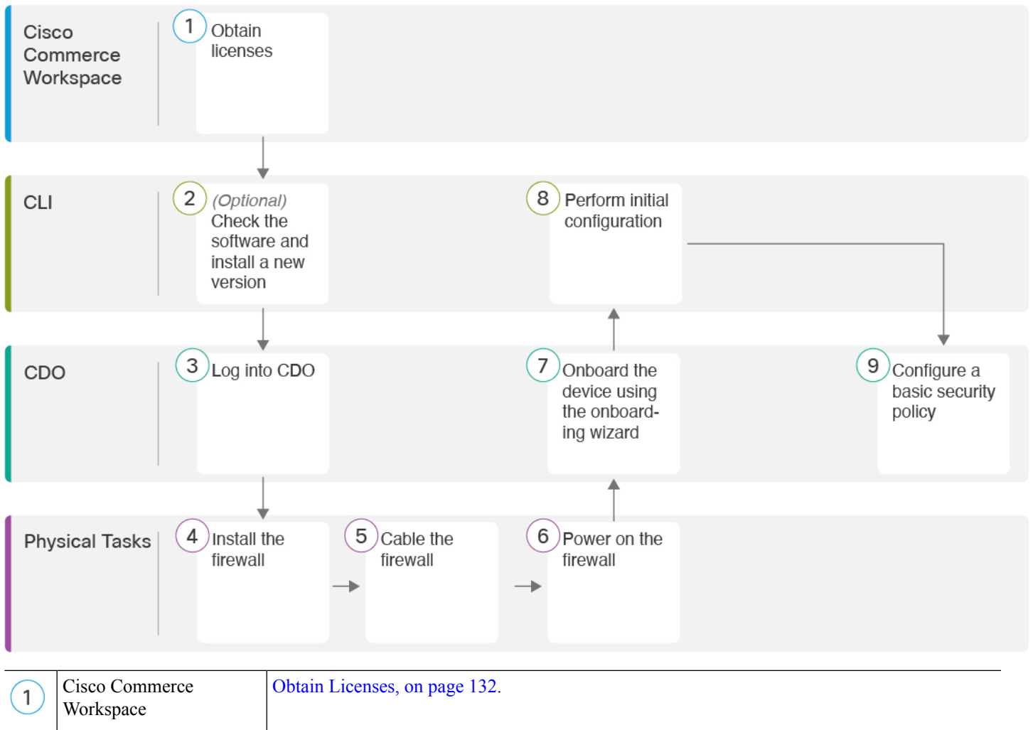
Figure 71: End-to-End Tasks: Onboarding Wizard
