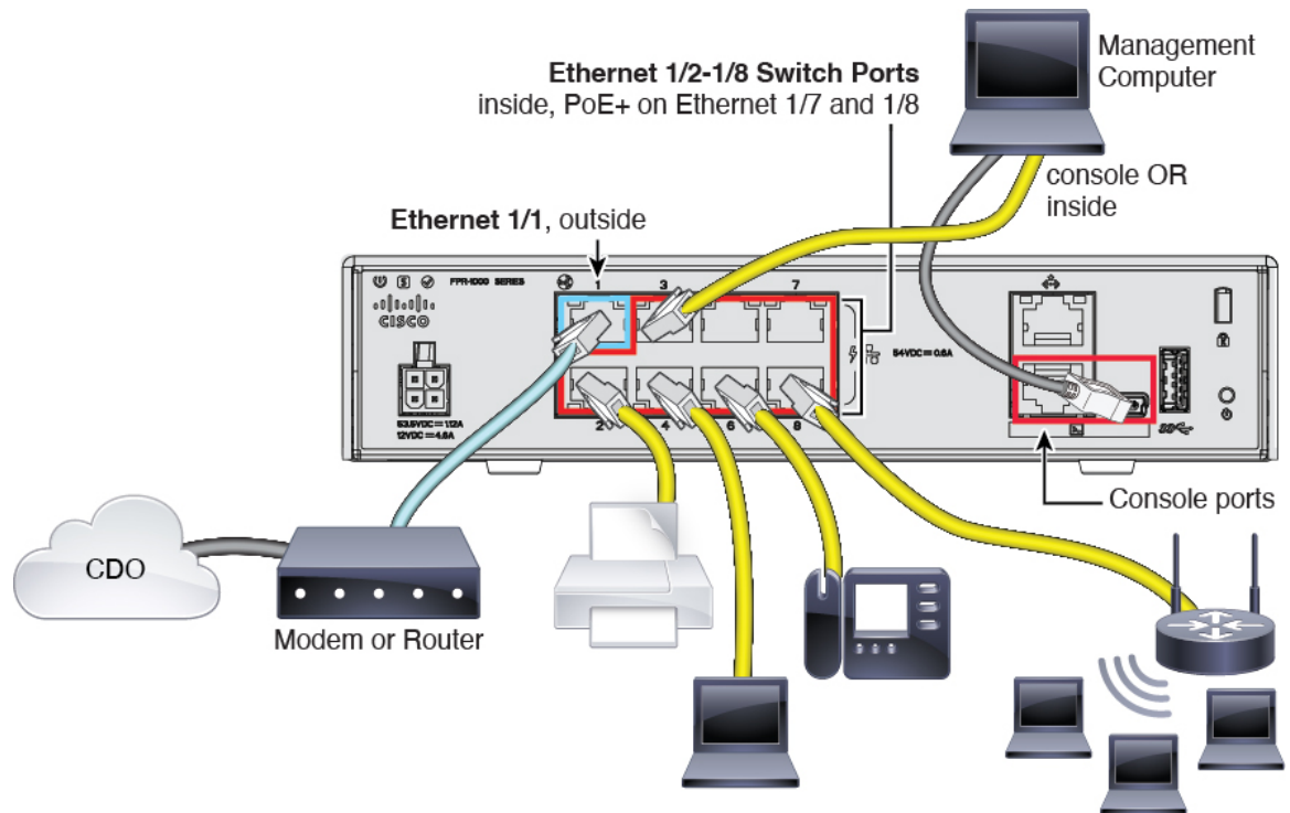
Figure 82: Cabling the Firepower 1010
