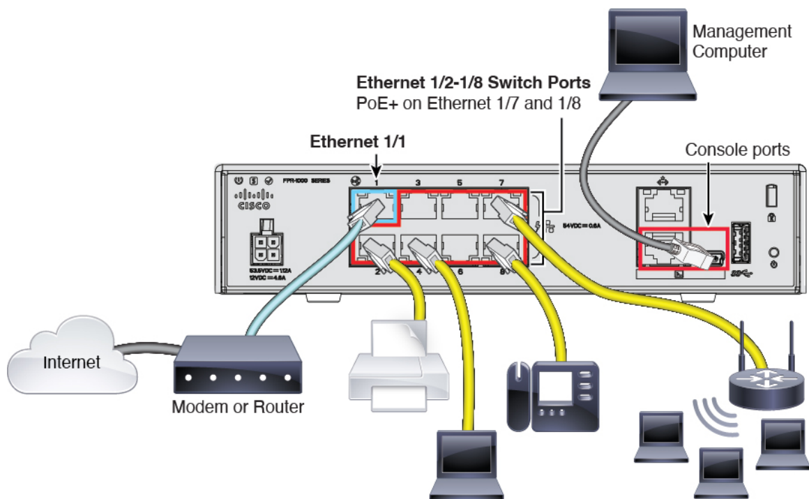
Figure 30: Cabling a Remote Management Deployment
