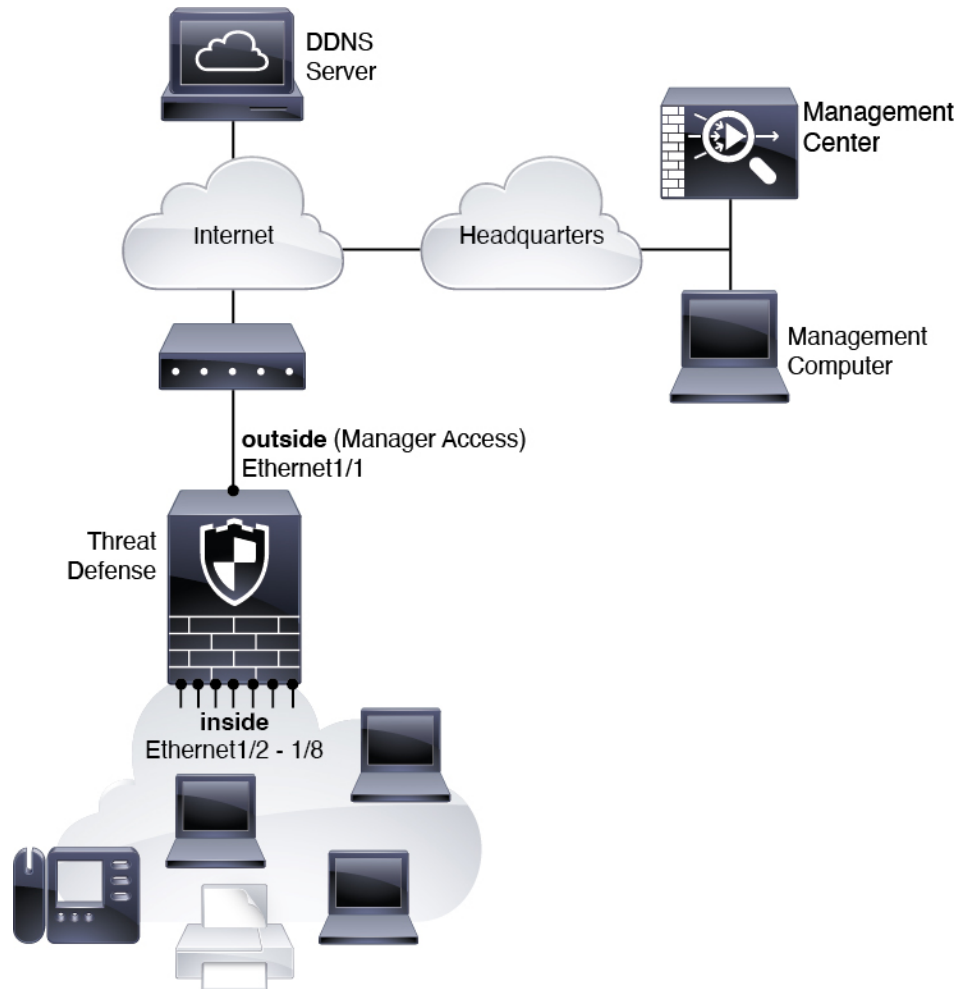
Figure 25: Manual Provisioning Network
