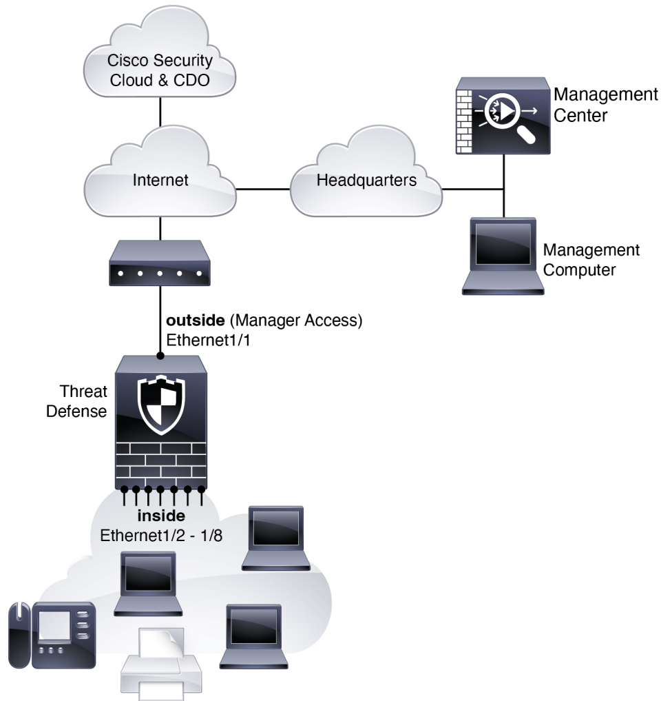
Figure 24: Zero-Touch Provisioning Network
