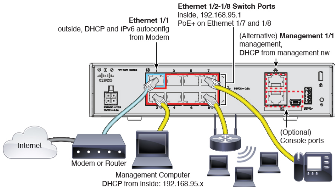
Figure 60: Cabling the Firepower 1010
