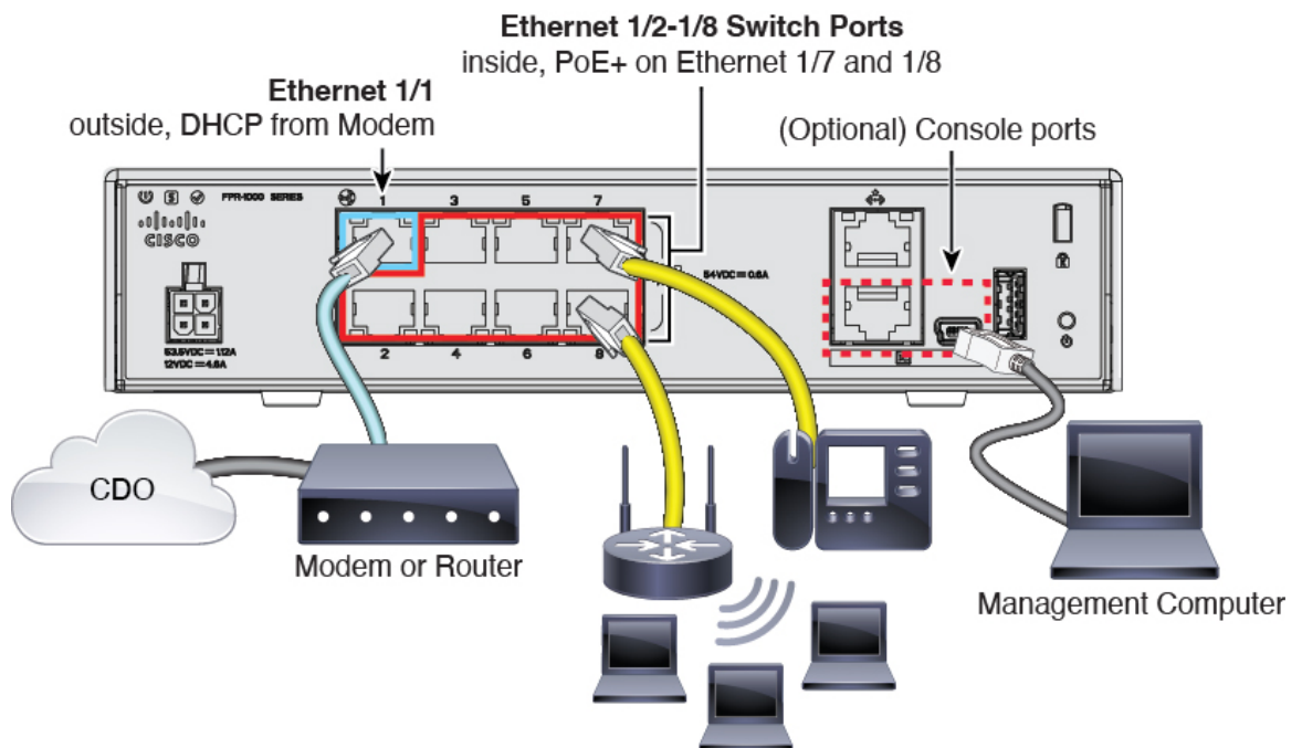
Figure 74: Cabling the Firepower 1010
