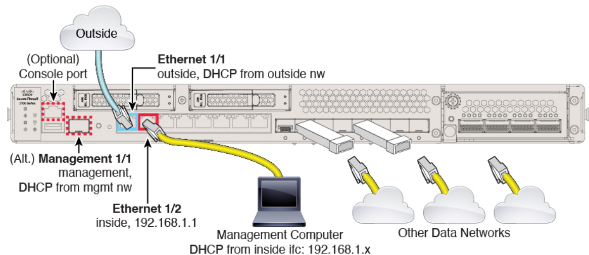
Figure 132: Cabling the Secure Firewall 3100
