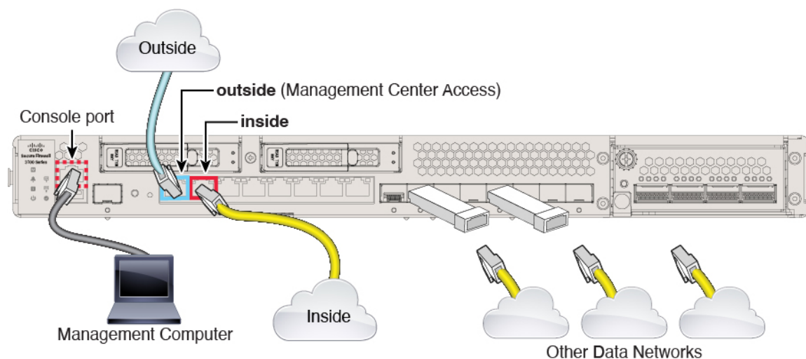
Figure 40: Cabling a Remote Management Deployment
