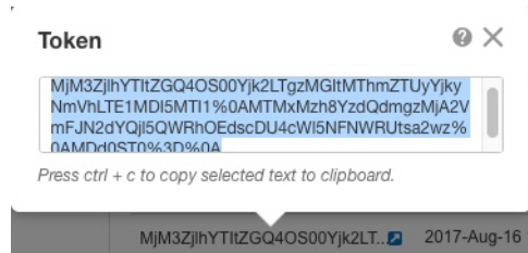
Figure 82: Copy Token
