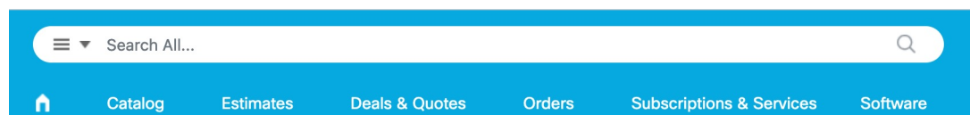
Figure 134: License Search
