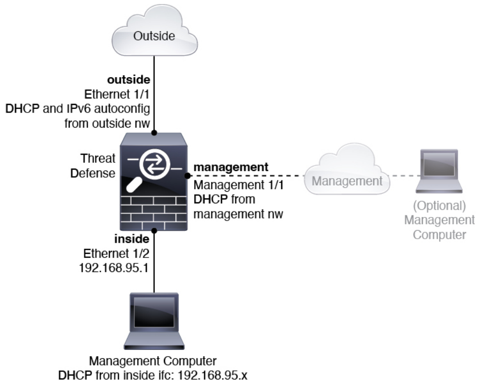
Figure 76: Suggested Network Deployment
