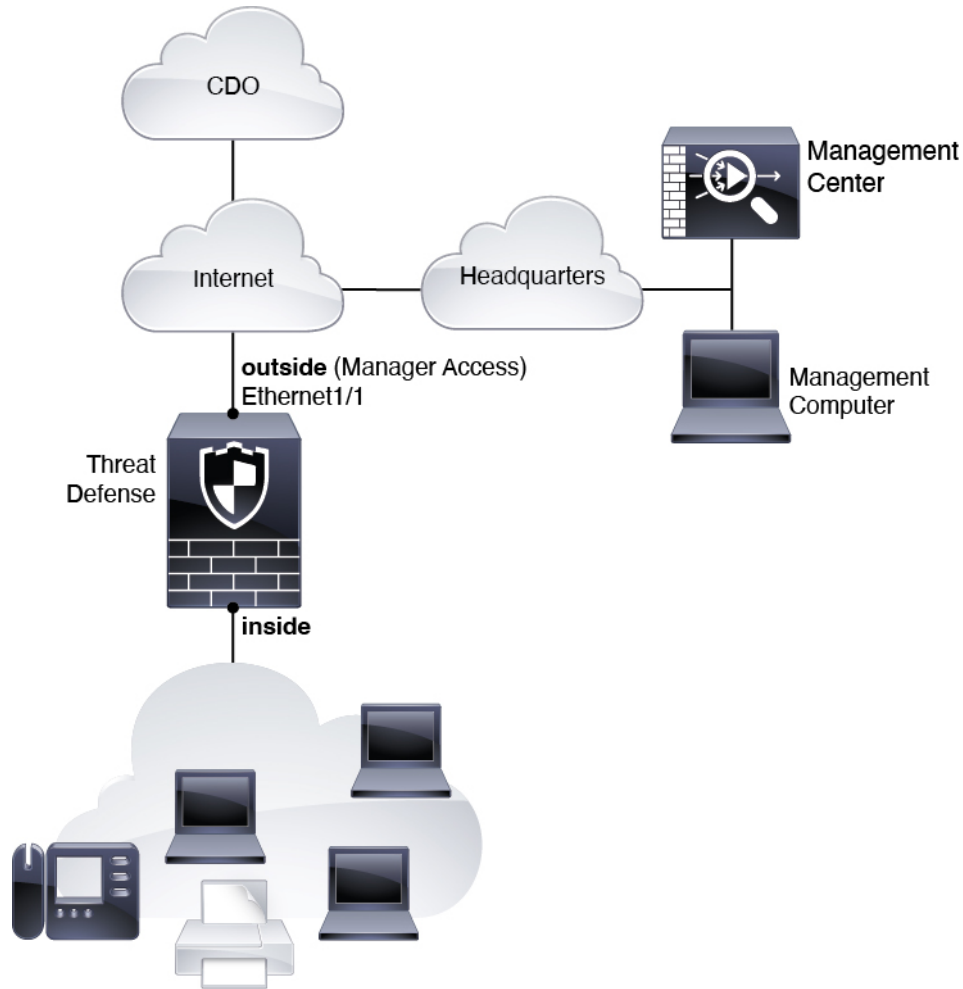
Figure 34: Zero-Touch Provisioning Network
