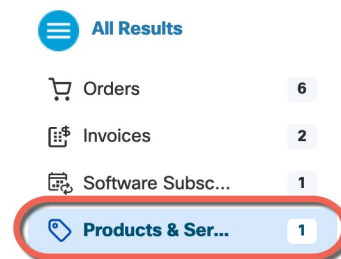
Figure 43: Results
