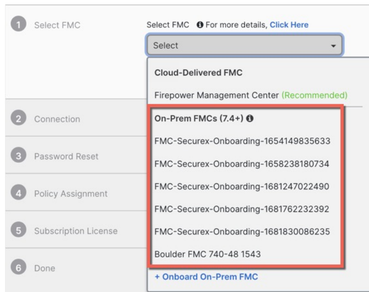
Figure 47: Select FMC
