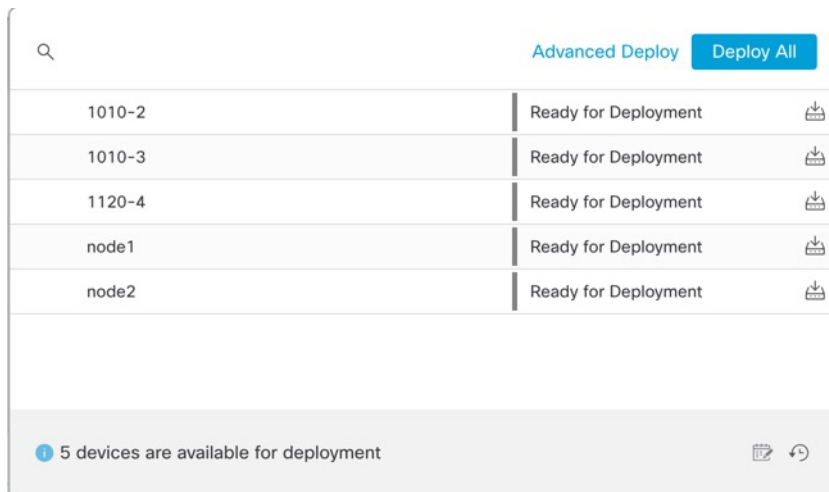
Figure 129: Advanced Deploy
