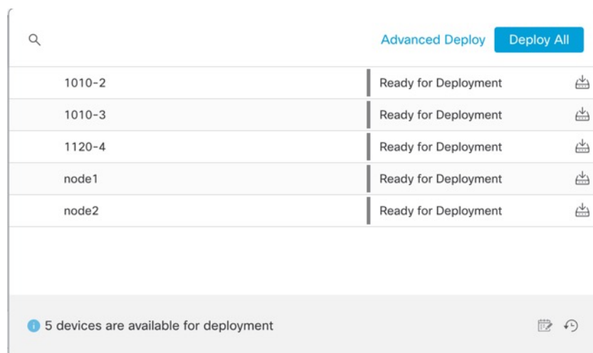
Figure 73: Advanced Deploy
