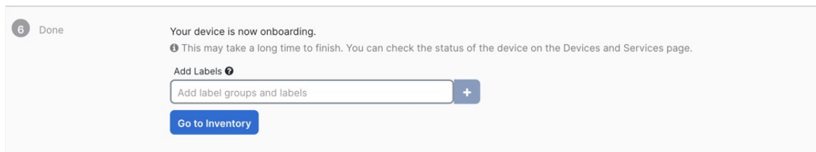
Figure 54: Done
