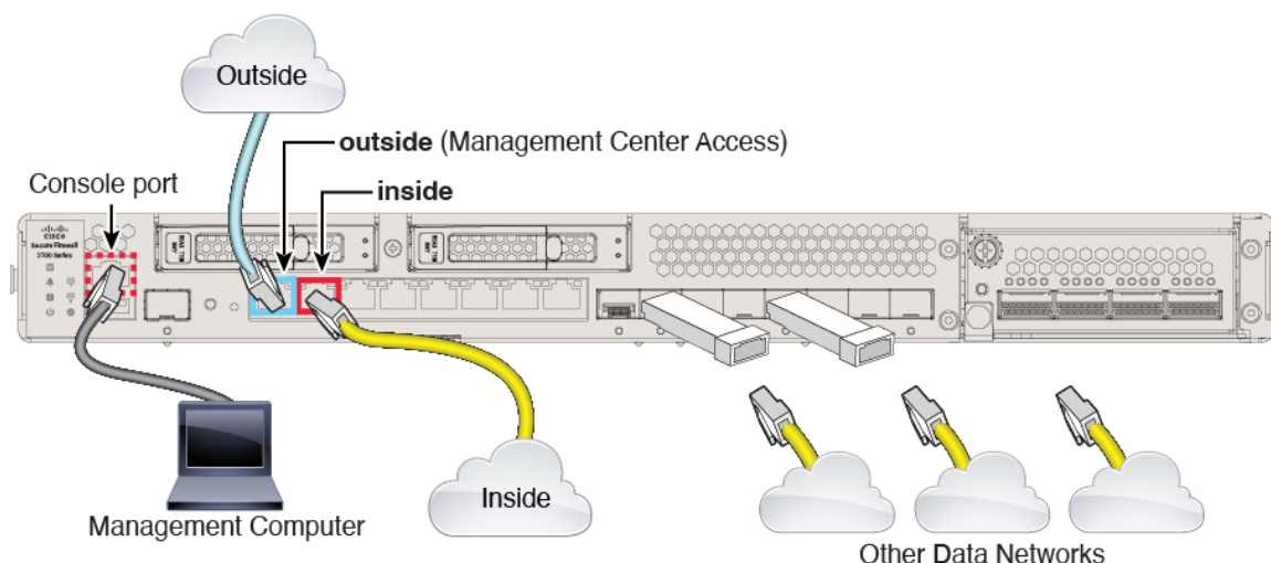
Figure 7: Cabling a Remote Management Deployment
