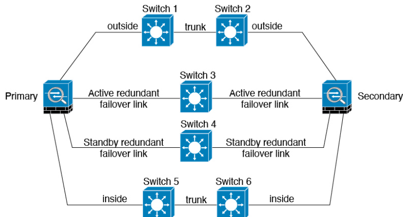
Figure 7: Connecting with Inter-switch Links
