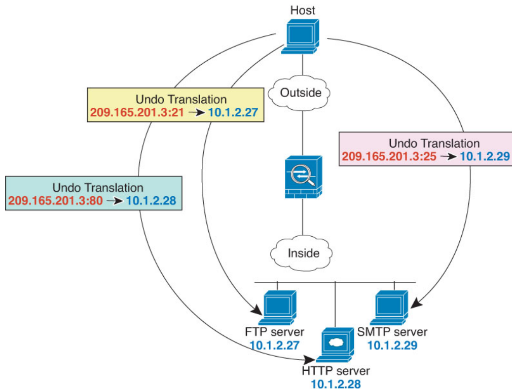
Figure 17: Static NAT-with-Port-Translation
