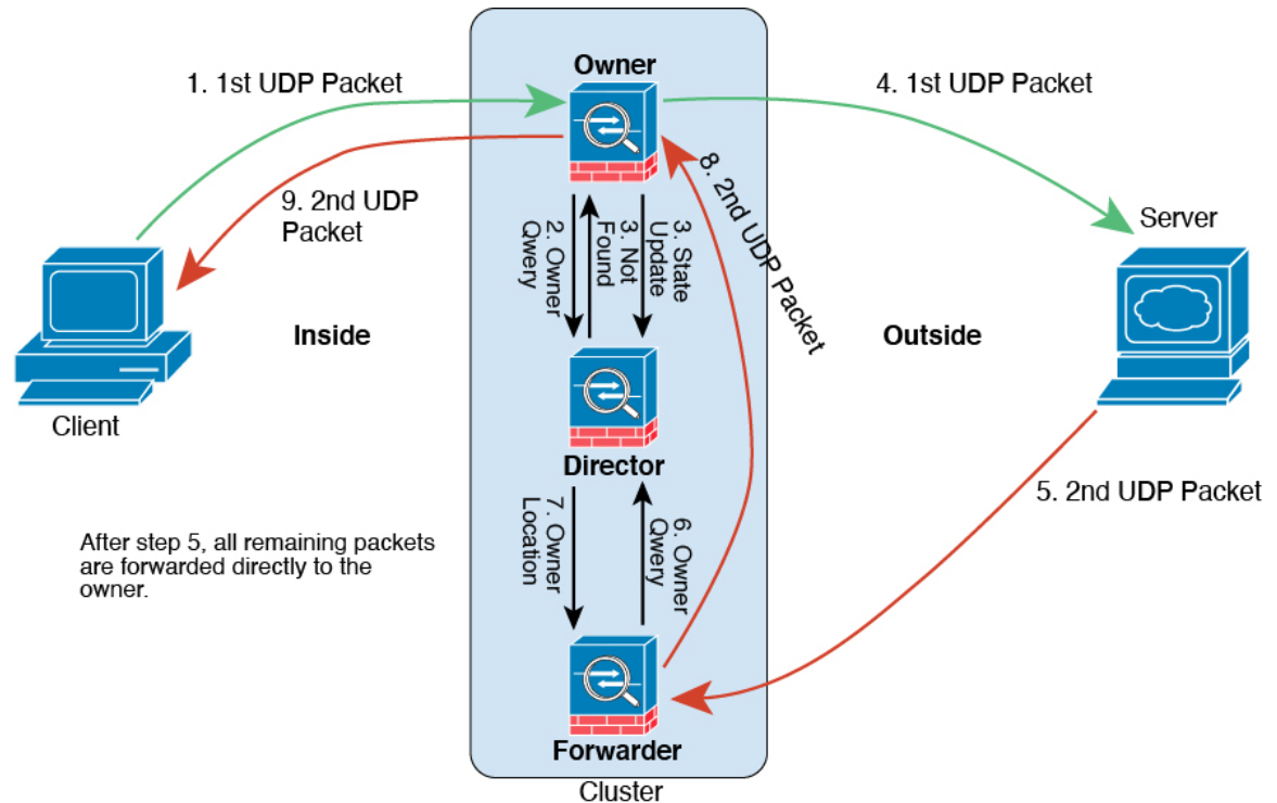
1. Figure 34: ICMP and UDP Data Flow
