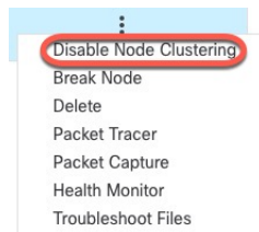
Figure 21: Disable Clustering
