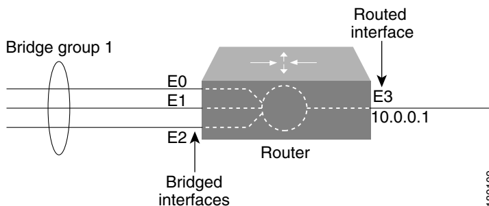
Figure 63-1 Transparent Bridging
