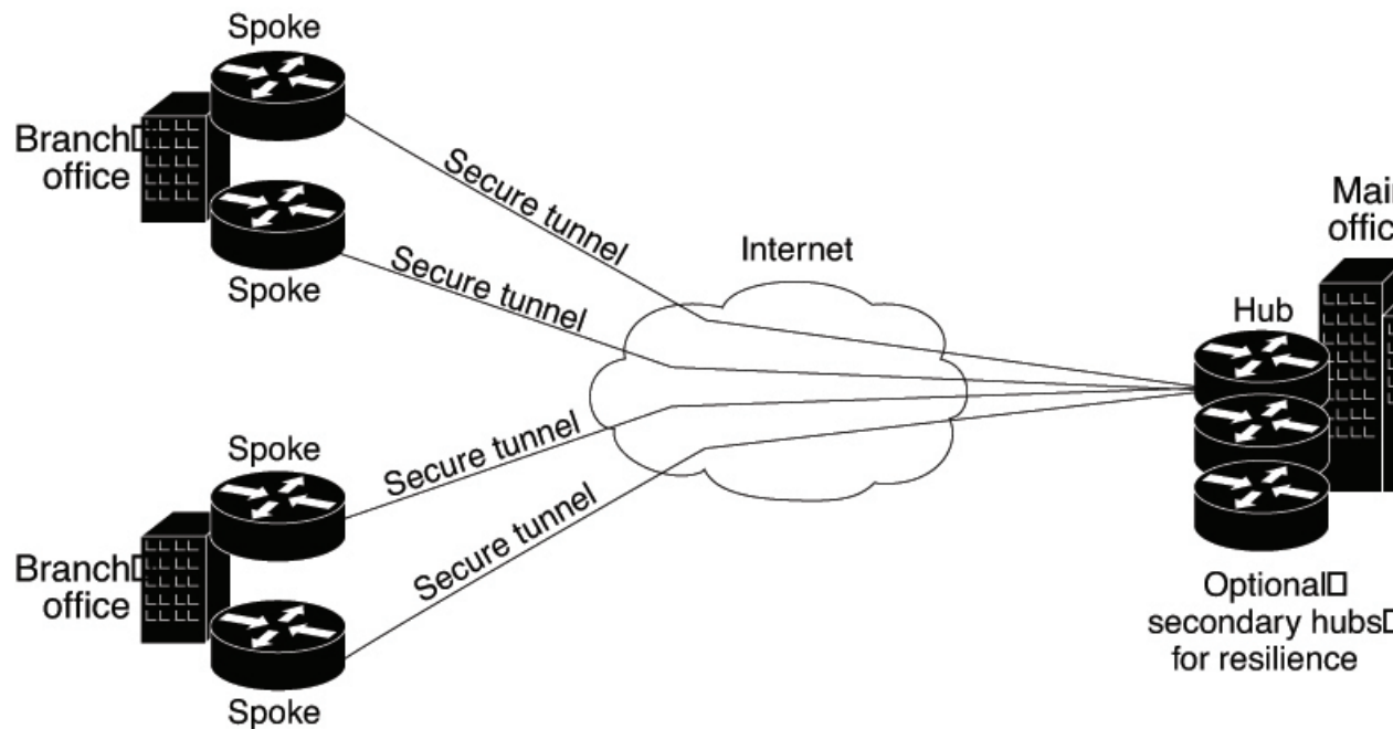
Figure 30: Hub-and-spoke VPN Topology
