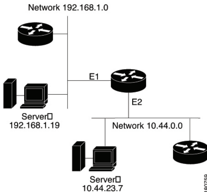
Figure 46: Helper Addresses
