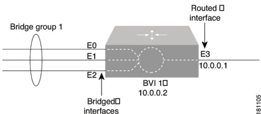
Figure 50: Bridge-Group Virtual Interface
