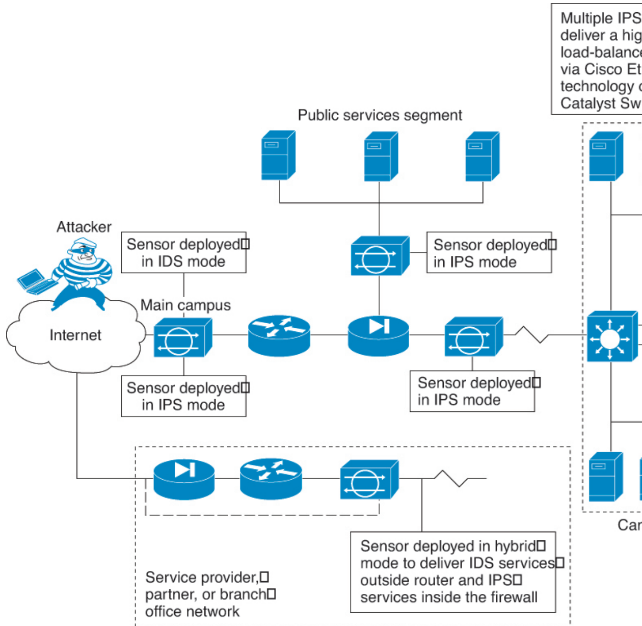
Figure 43: Comprehensive IPS Deployment Solutions
