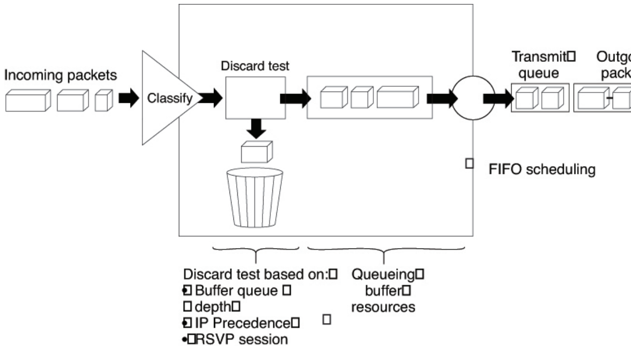
Figure 54: Weighted Random Early Detection
