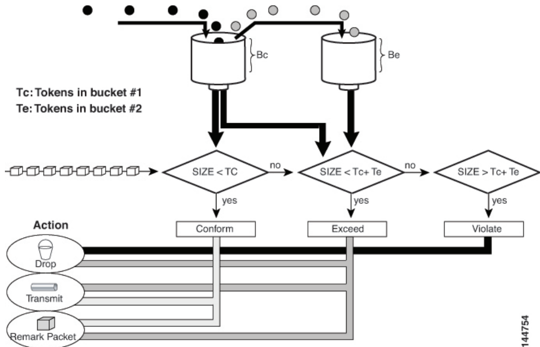
Figure 56: Two-Token Bucket Algorithm
