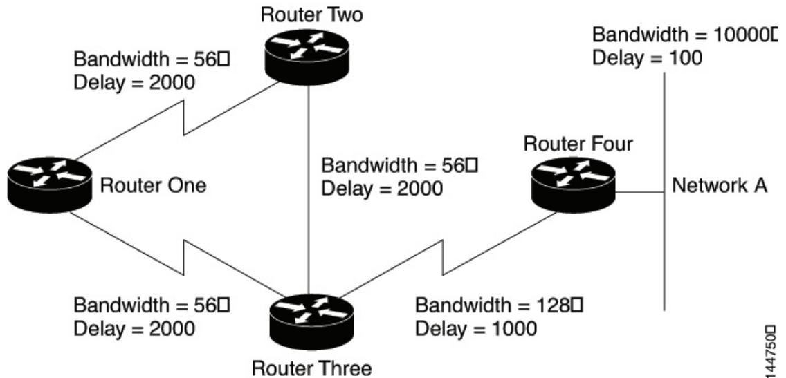
Figure 57: EIGRP Split Horizon Example
