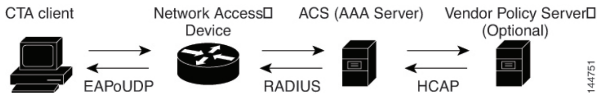
Figure 53: NAC System Flow
