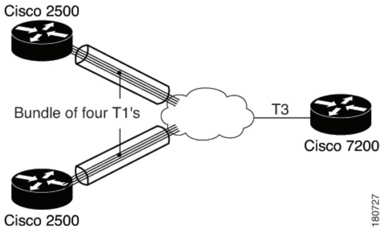
Figure 48: Multilink PPP
