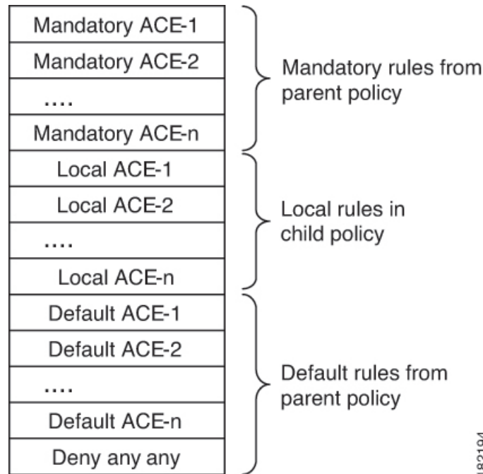
Figure 2: Order of Rules When Using Inheritance
