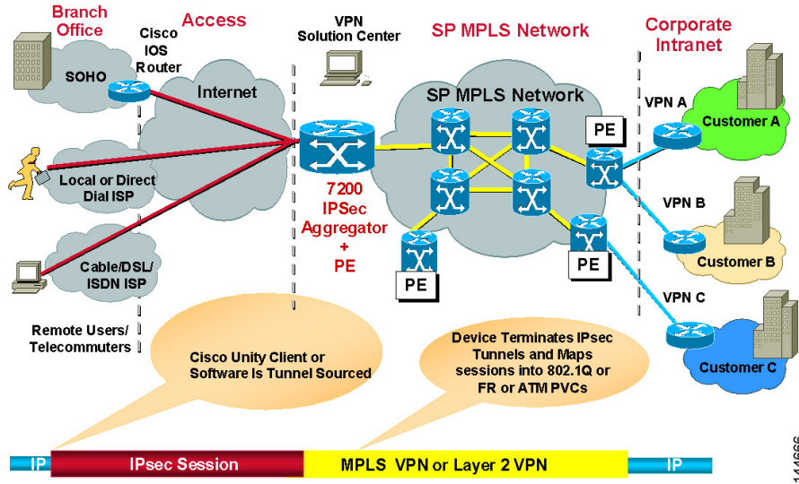
Figure 36: VRF-Aware IPsec One-Box Solution
