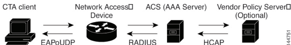
Figure 53: NAC System Flow
