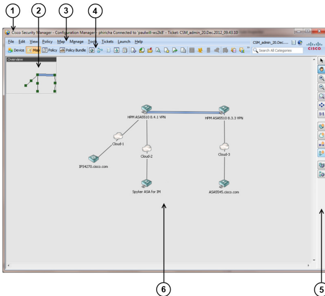
Figure 3: Map View Overview
