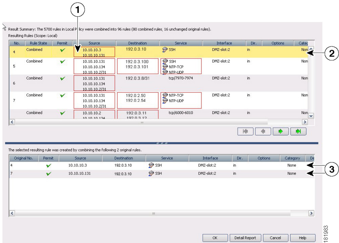
Figure 19: Example of Rule Combiner Results
