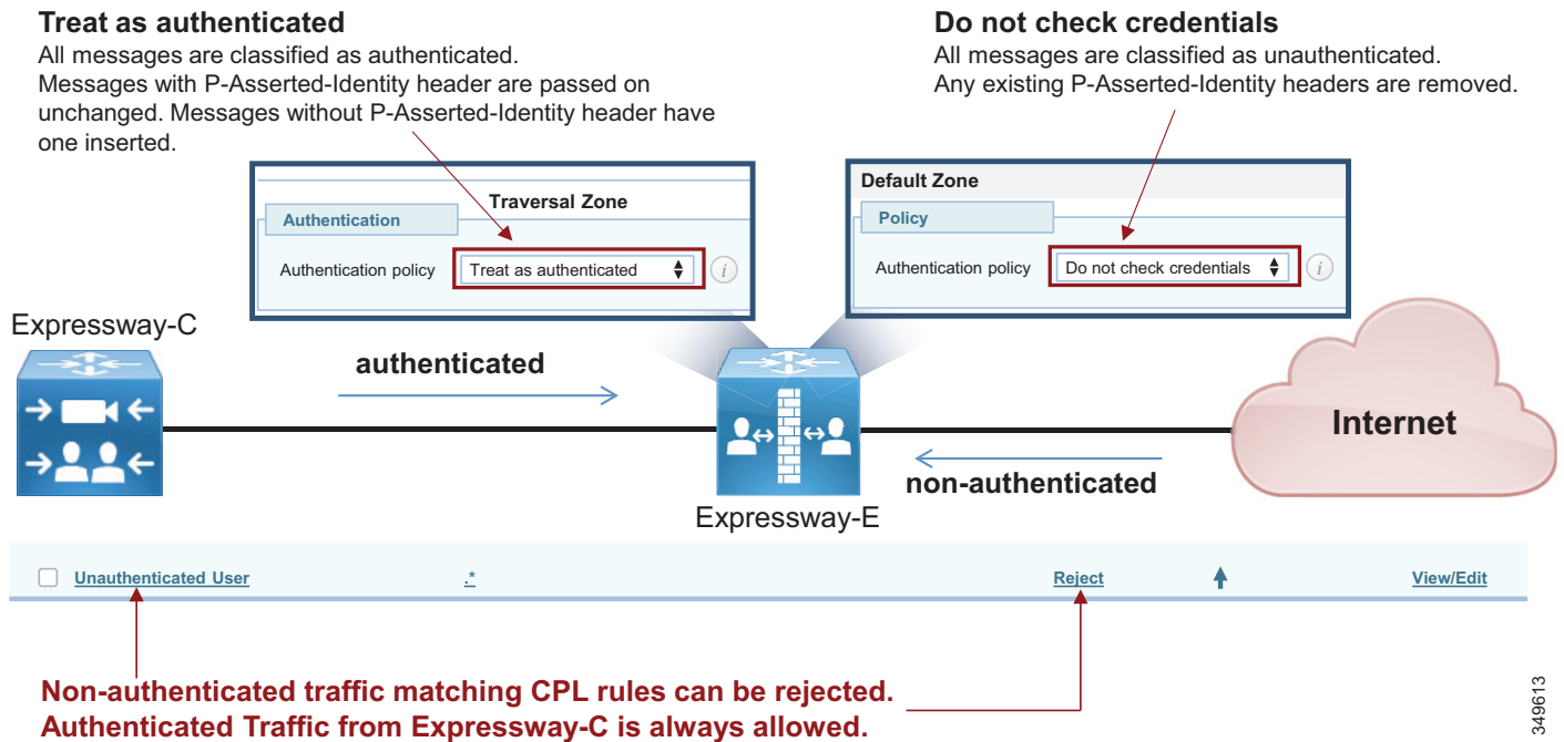
Figure 4-17 Call Authentication
