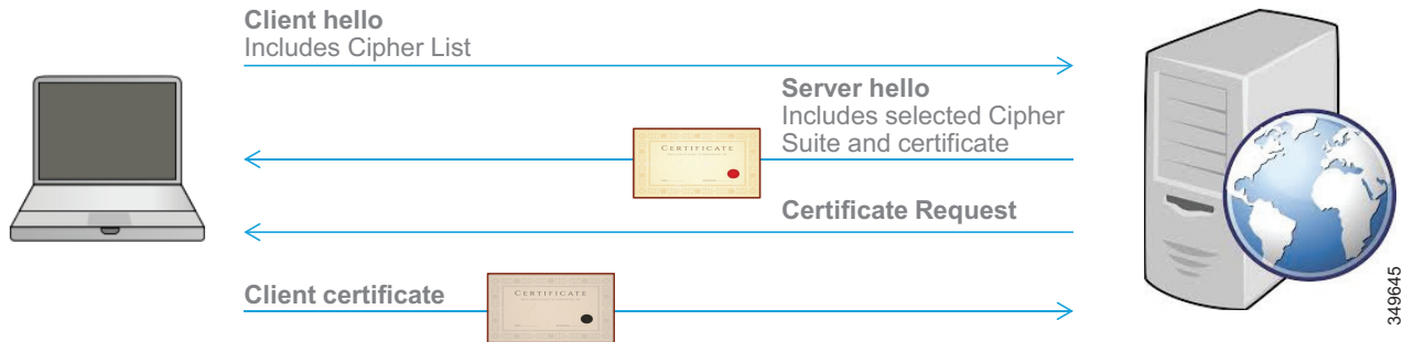
Figure 7-5 MTLS Handshake
