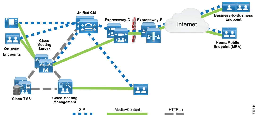
Figure 3-5 Standard Deployment
