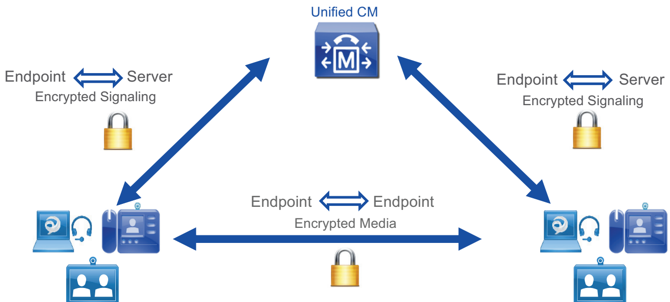
Figure 7-6 Signaling and Media Encryption with Unified CM Registered Endpoints
