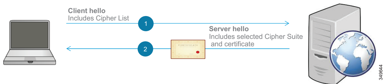
Figure 7-4 TLS Handshake
