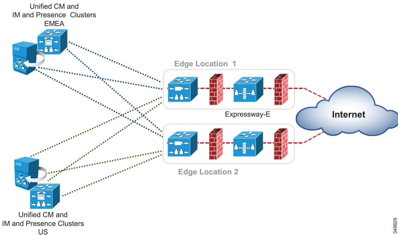
Figure 4-18 Service Discovery of Multiple Unified CM and IM and Presence Clusters
