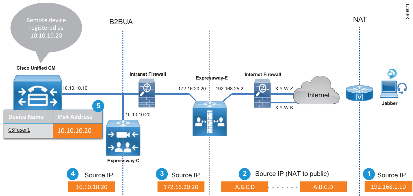
Figure 4-7 NAT in the Life of a Packet
