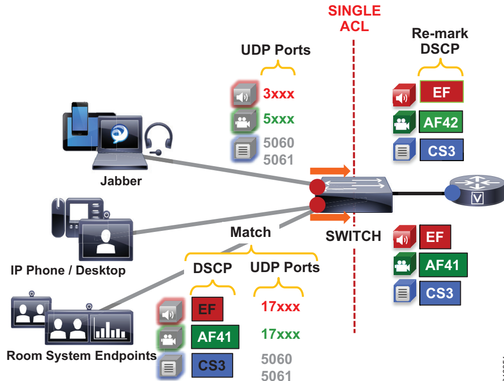
Figure 8-8 Endpoint Marking
