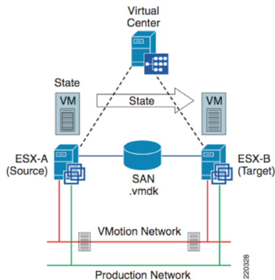
Figure 2-14 vMotion Process
