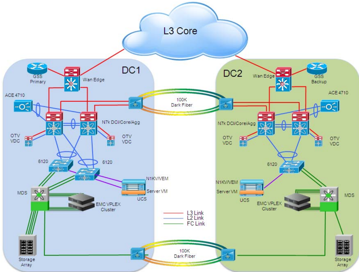
Figure 2-32 EMC VPLEX Metro Deployment
