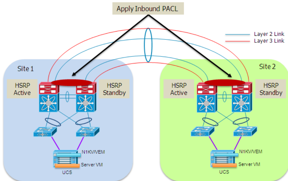
Figure 2-7 HSRP Isolation across the vPC Connection
