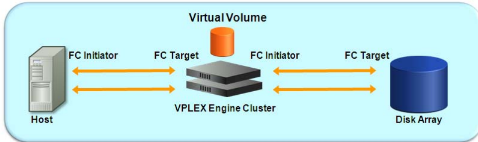
Figure 2-29 Initiator and Target Roles with VPLEX
