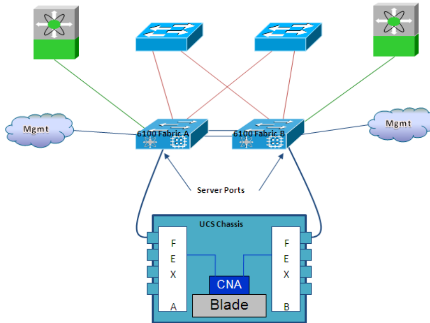
Figure 2-20 UCS Connections
