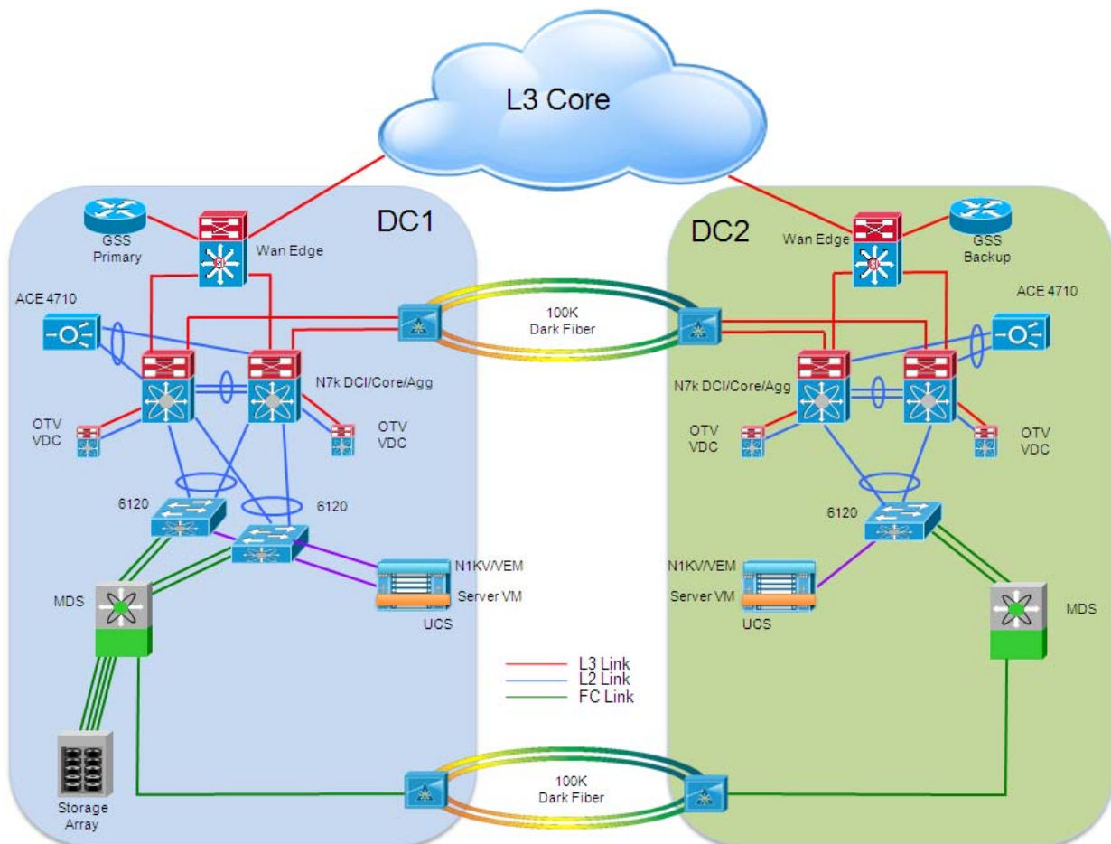
Figure 2-27 FC Access to Shared Storage
