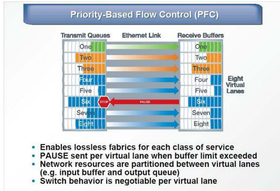
Figure 2-57 Priority Flow Control
