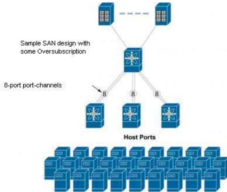
Figure 2-53 SAN Design
