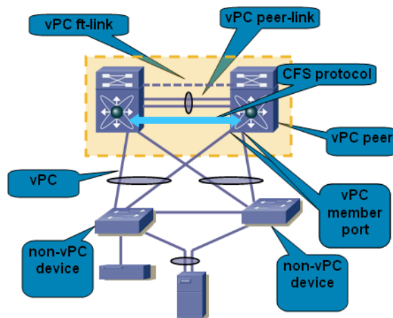
Figure 2-26 vPC Design
