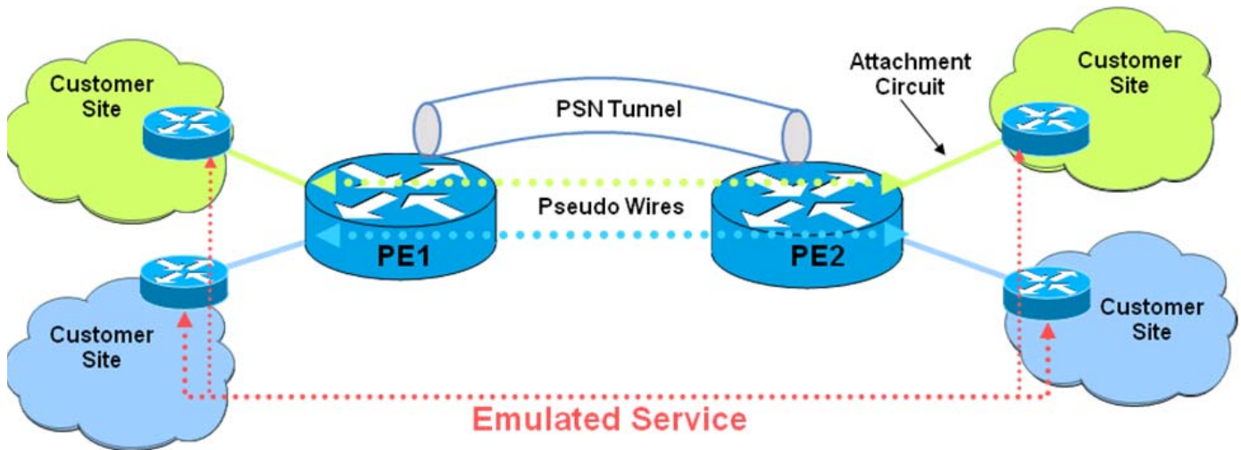
Figure 2-41 Pseudowire Reference Model
