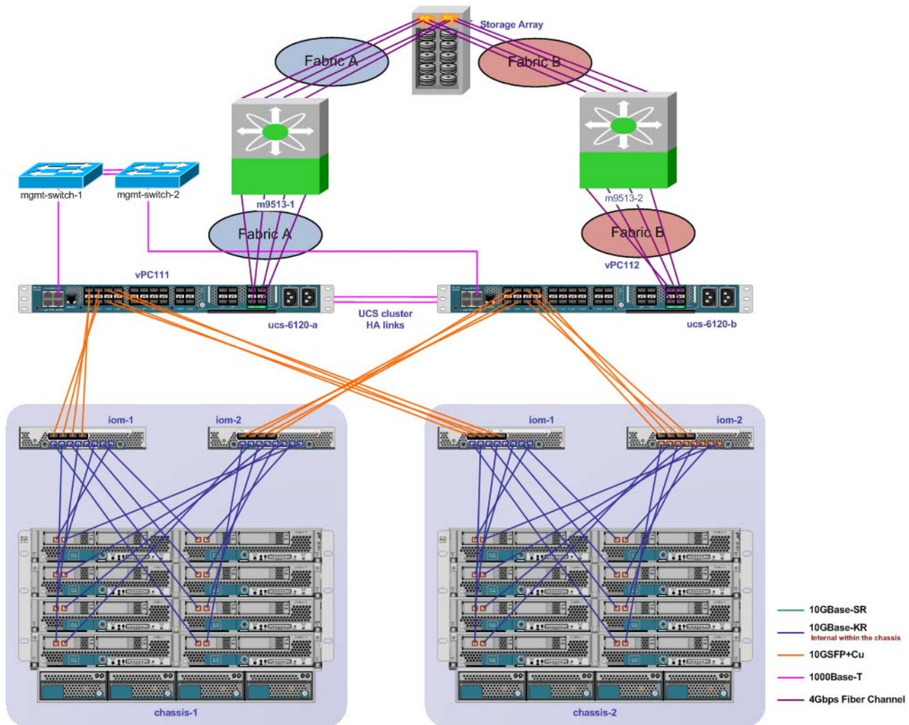
Figure 2-20 SAN Layout
