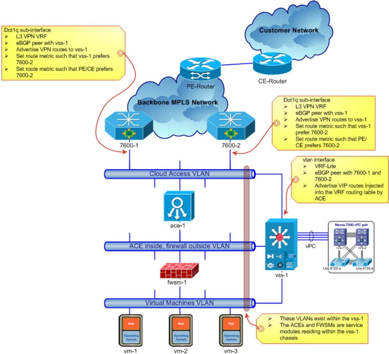
Figure 2-38 Gold Service Class L3VPN Setup
