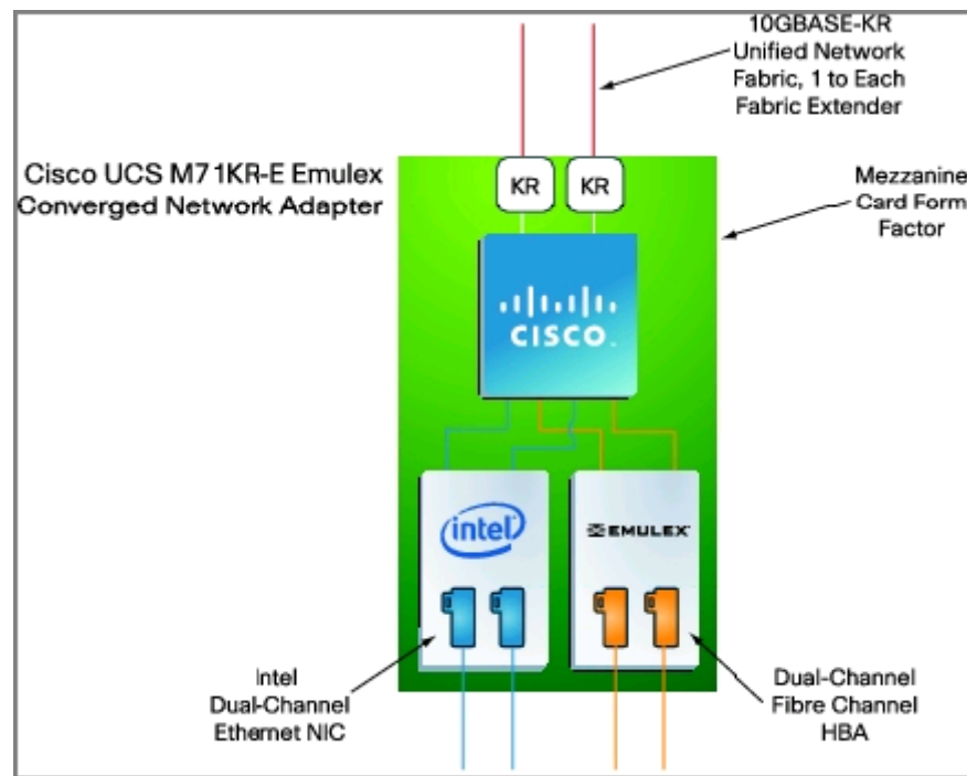
Figure 2-7 UCS M71KR-E Adapter
