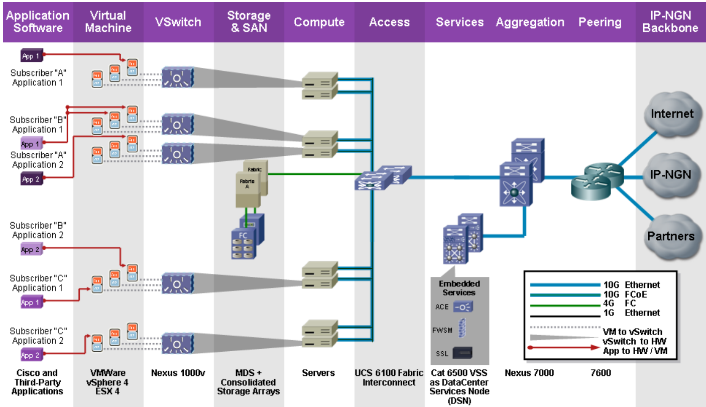
Figure 1-1 Solution Architecture
