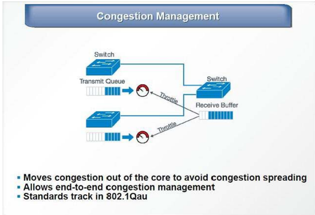
Figure 2-60 Congestion Notification IEEE 802.1Qau (Future)
