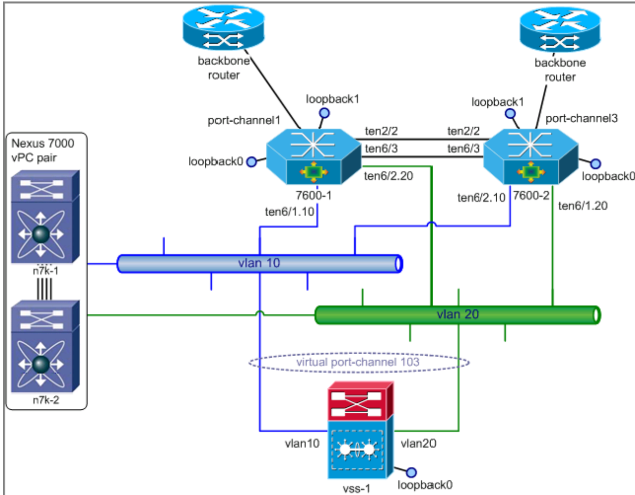
Figure 2-36 Logical IP Network Setup
