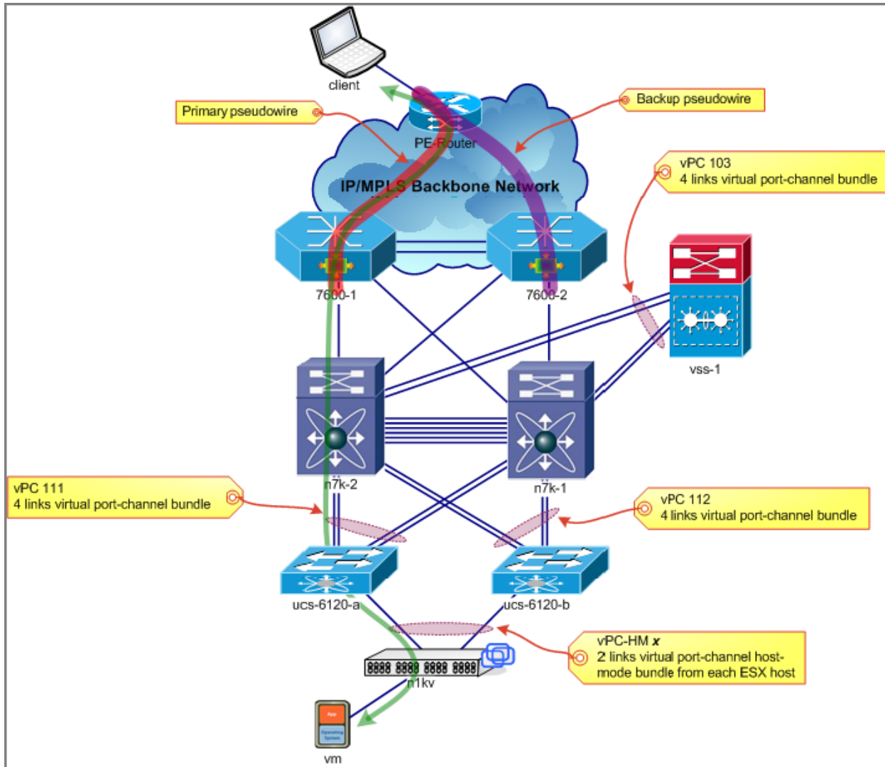
Figure 2-49 L2VPN Bronze Service Class Data Traffic
