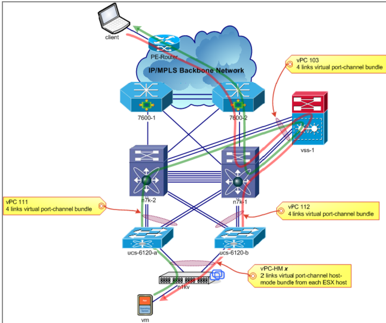
Figure 2-46 L3VPN Gold and Silver Service Classes Data Traffic
