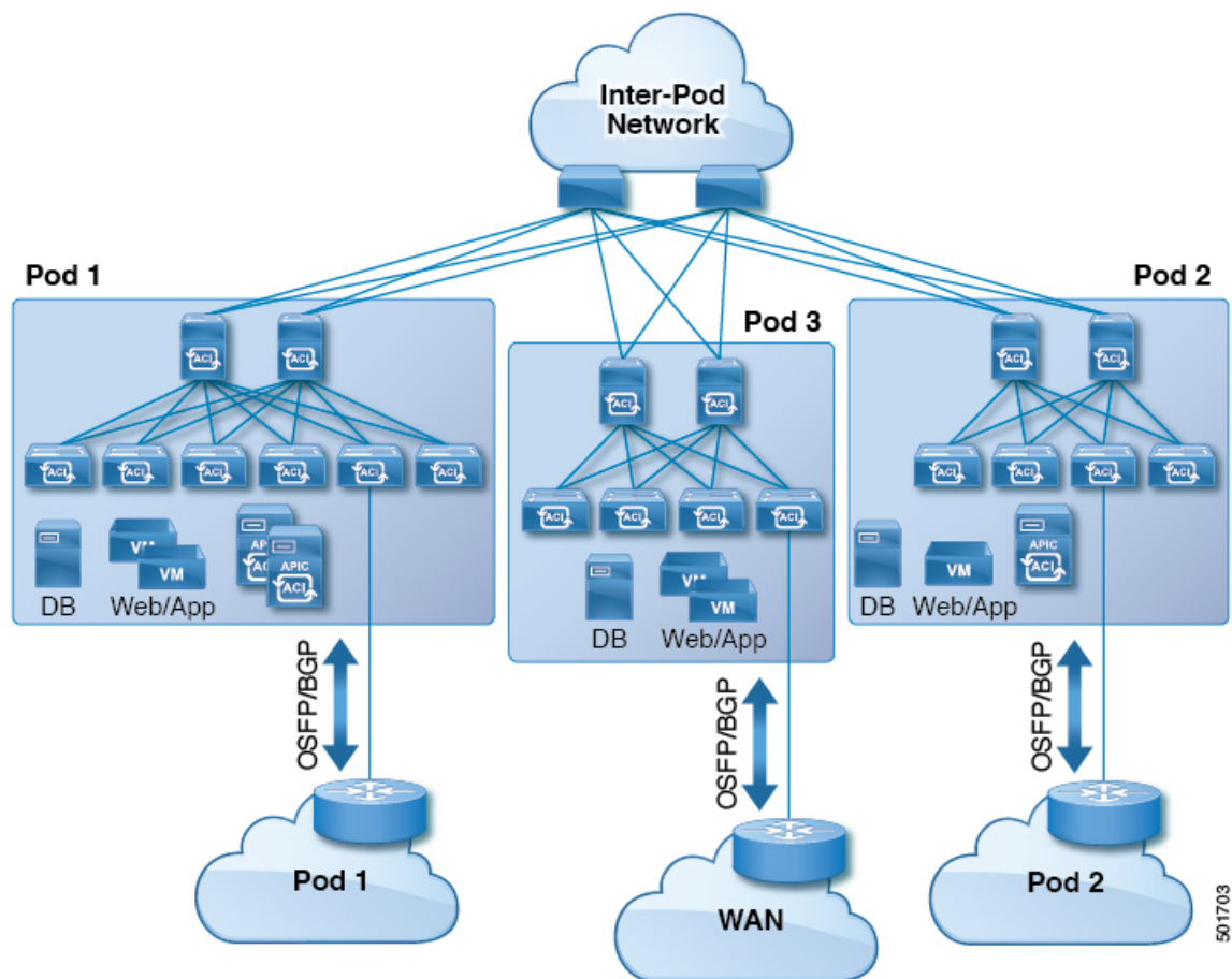
Figure 35: Multiple Pods with L3Outs in a Transit-Routed Configuration
