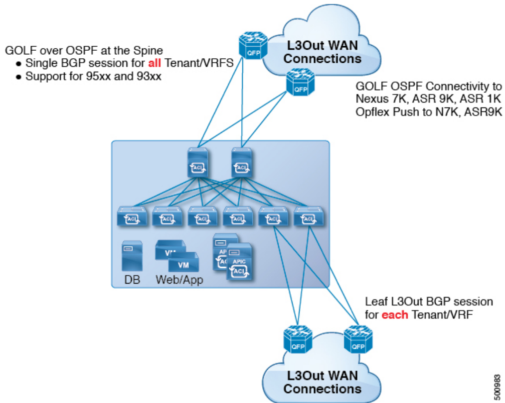
Figure 27: Cisco ACI GOLF Topology
