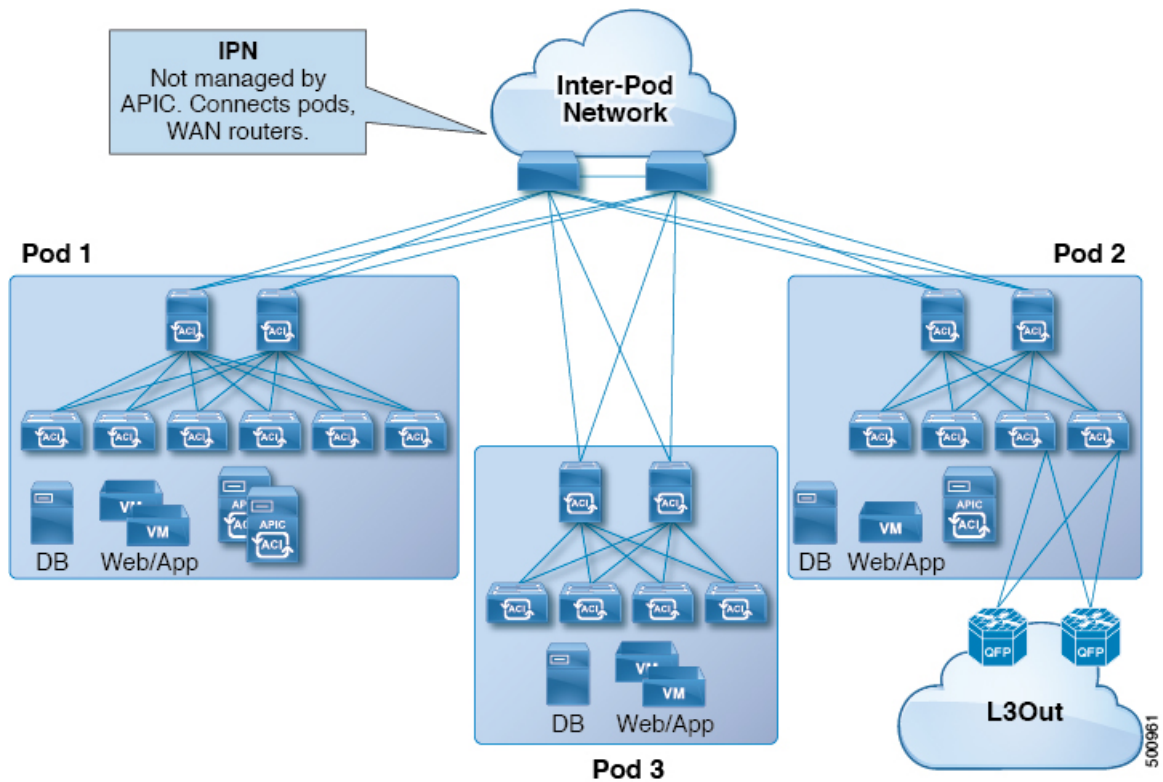
Figure 28: Multi-Pod Overview
