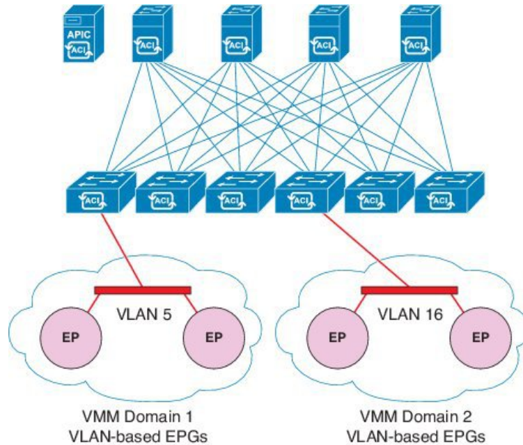
Figure 93: VMM Domain EPG VLAN Consumption
