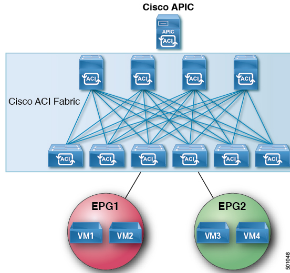
Figure 49: VM1 to VM2 Communication is Desired.
