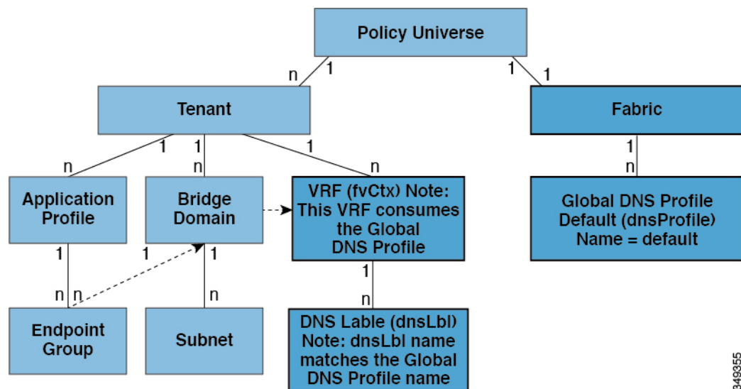
Figure 58: DNS
