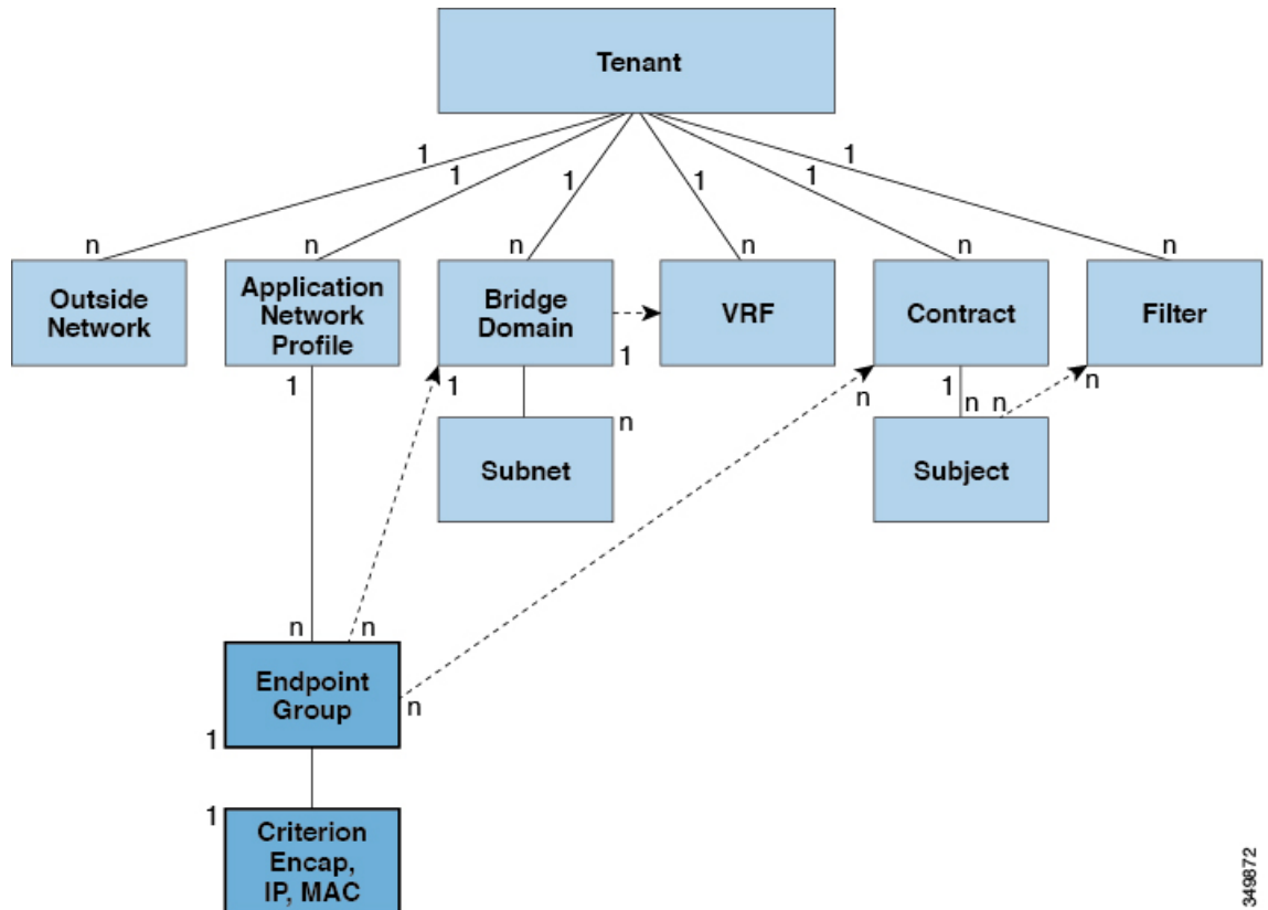
Figure 9: Endpoint Groups
