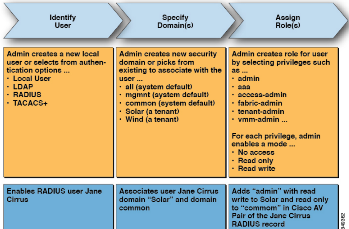
Figure 89: Process for Configuring Users on External Authentication Servers
