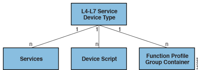
Figure 95: Layer 4 to Layer 7 Policy Model
