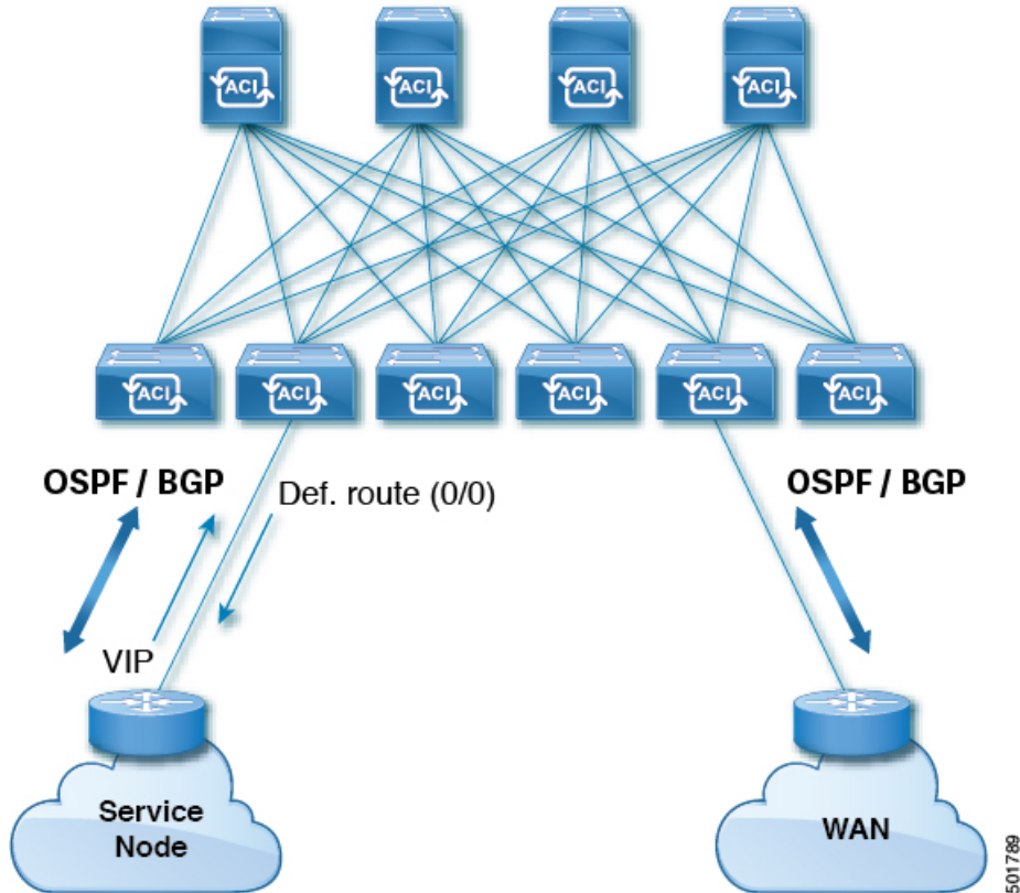
Figure 82: Service Node Transit Connectivity
