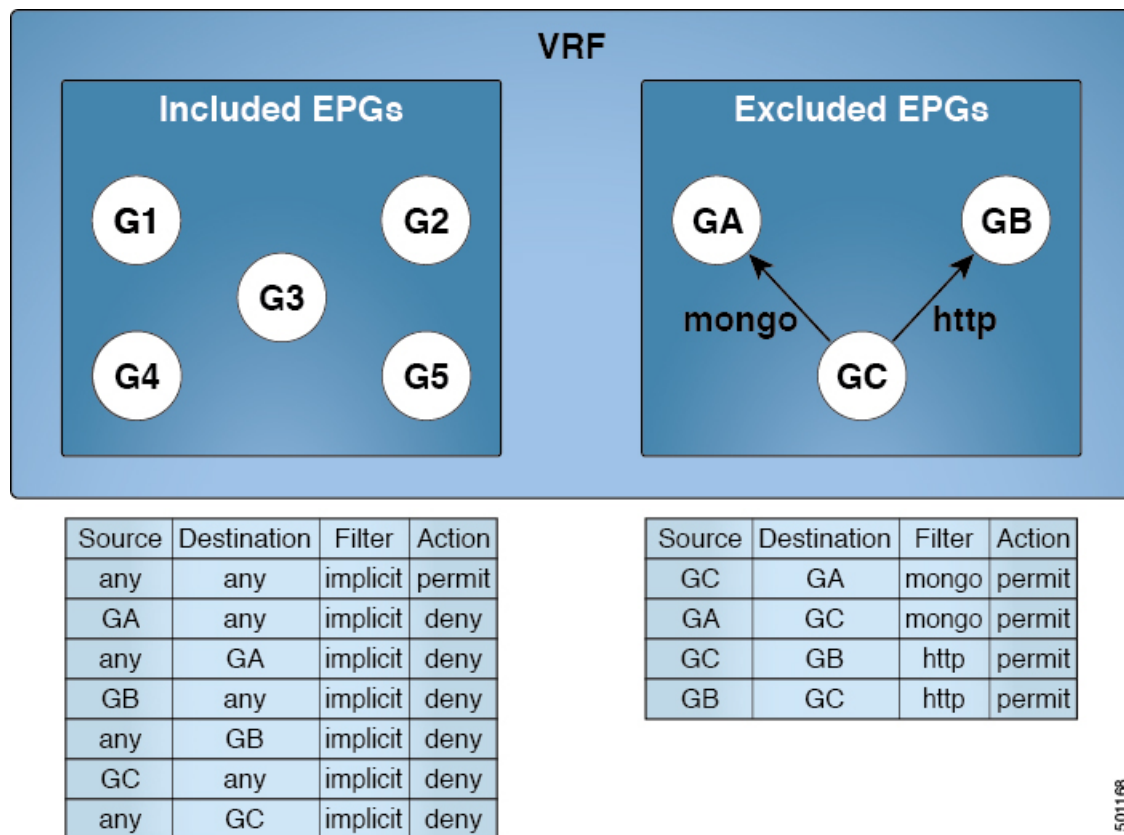
Figure 18: Contract Preferred Group Overview
