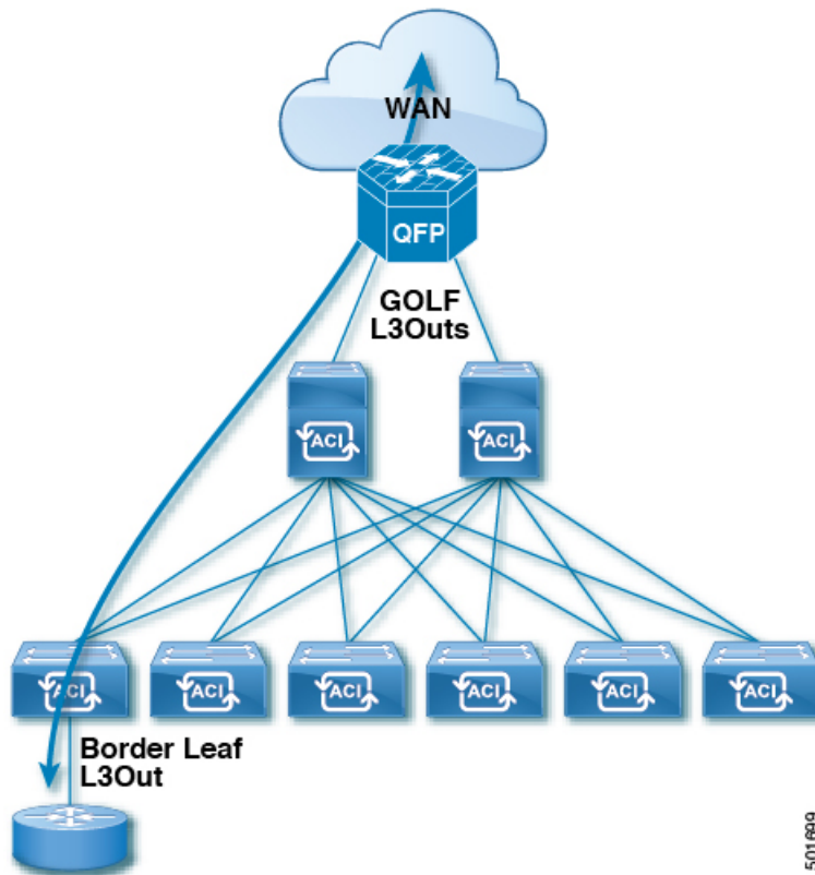
Figure 84: GOLF L3Outs and a Border Leaf L3Out in a Transit-Routed Configuration
