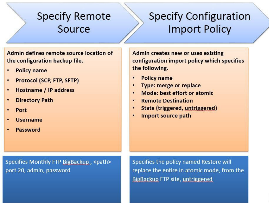
Figure 118: Workflow for Configuring an Import Policy
