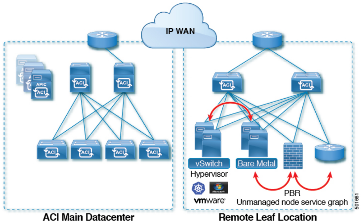
Figure 77: Remote Leaf Topology
