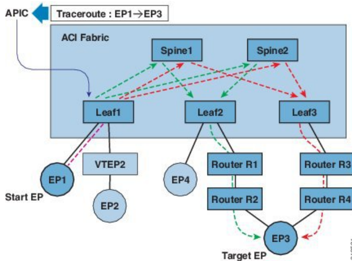
Figure 126: APIC Endpoint to Endpoint Traceroute
