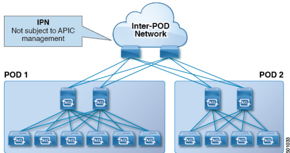
Figure 78: Multipod Topology
