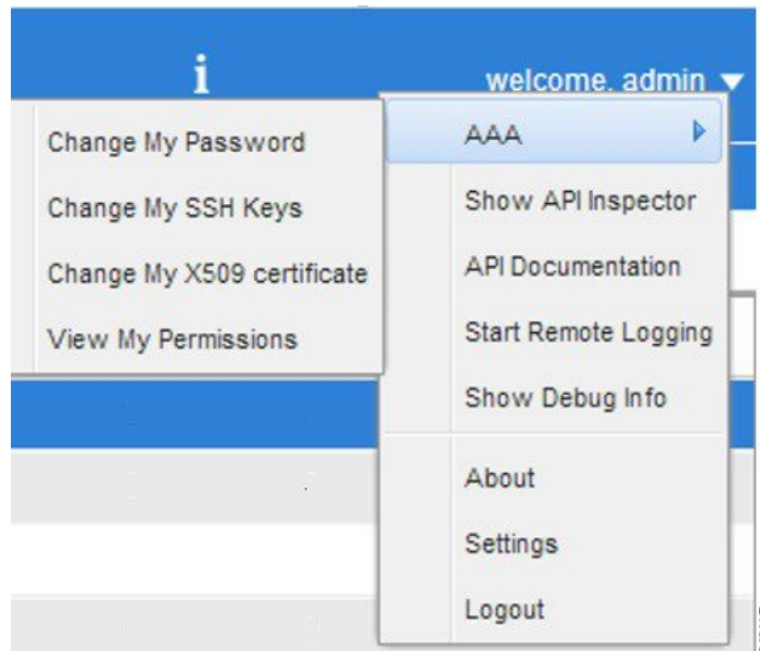
Figure 108: User Login Menu Options
