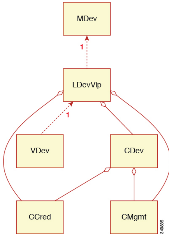
Figure 105: Managed Object Model Without a Device Manager or Chassis Manager
