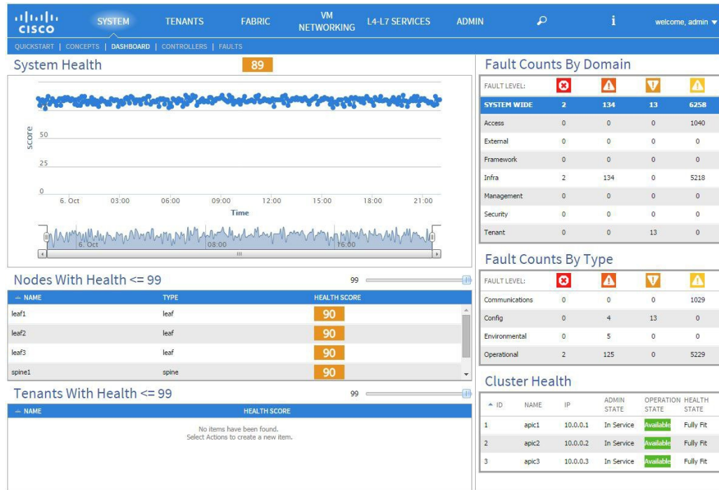
Figure 127: System Health Scores
