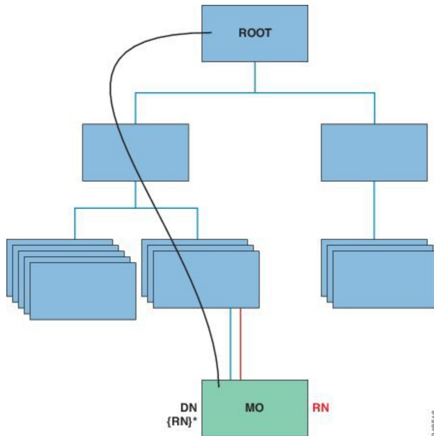
Figure 112: MO Distinguished and Relative Names
