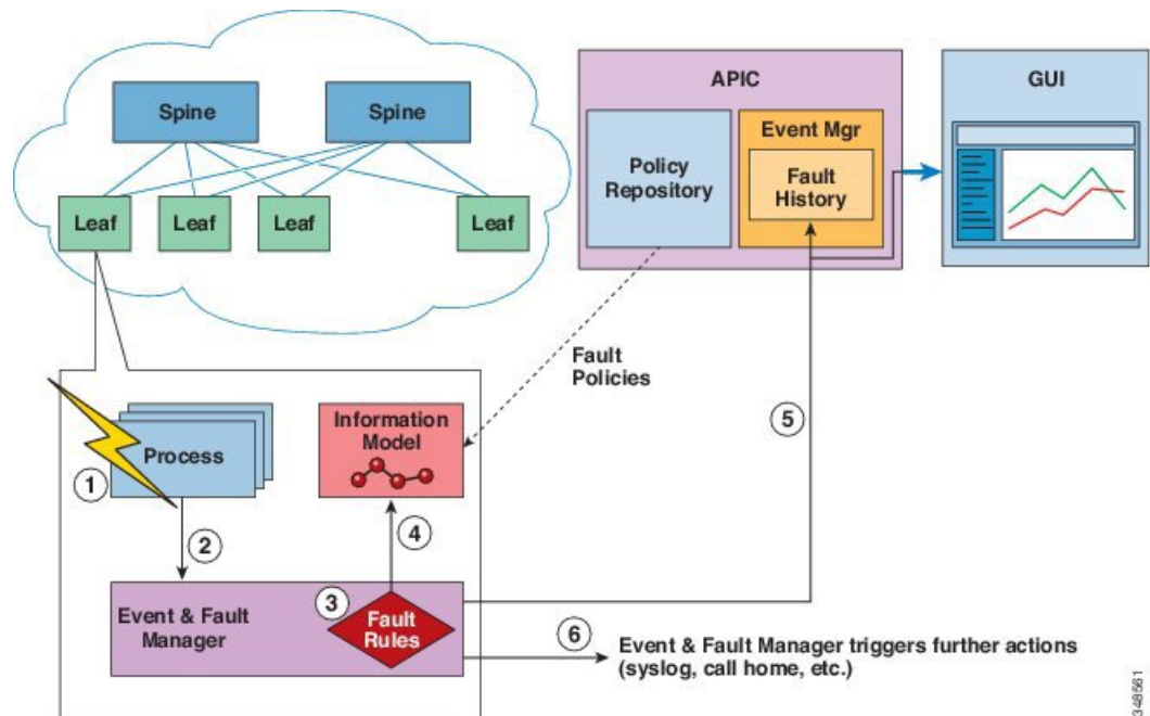
Figure 120: Faults and Events Reporting/Export
