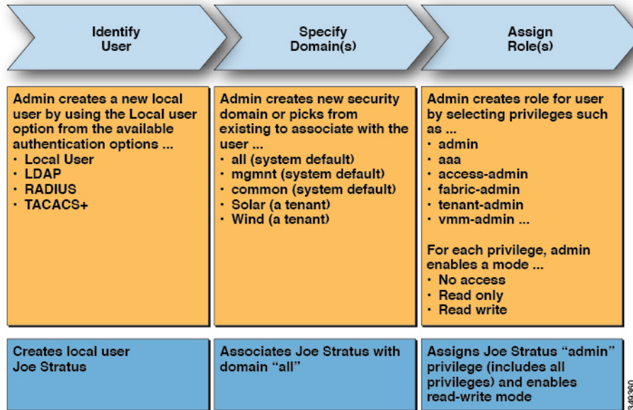
Figure 87: APIC Local User Configuration Process
