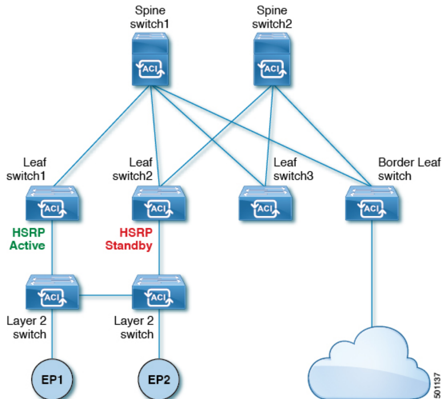
Figure 79: HSRP Deployment Topology
