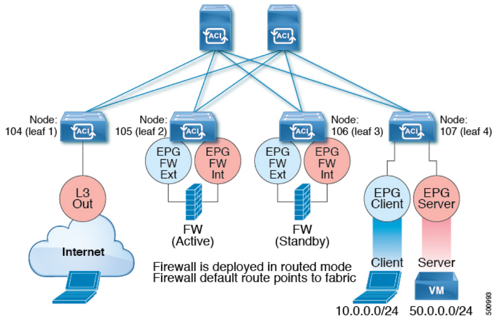
Figure 99: Sample ACI PBR Physical Topology
