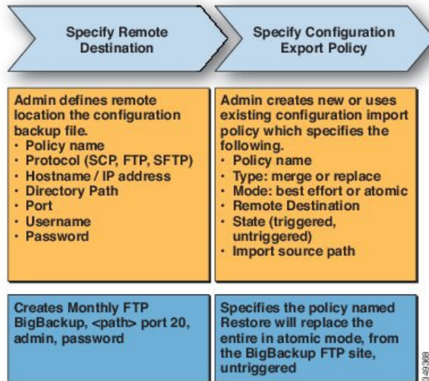
Figure 117: Workflow for Configuring an Export Policy
