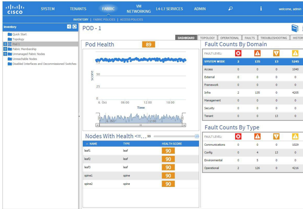
Figure 128: Pod Health Scores
