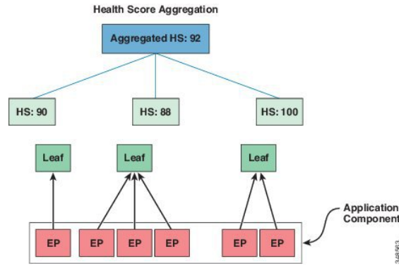
Figure 132: Health Score Aggregation
