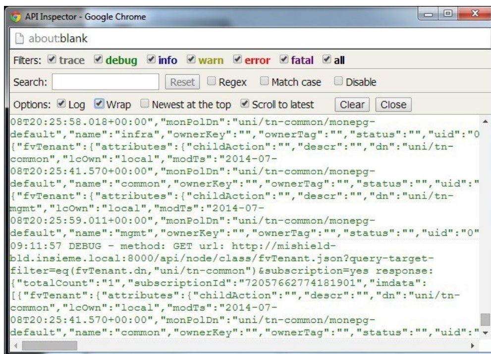
Figure 109: API Inspector
