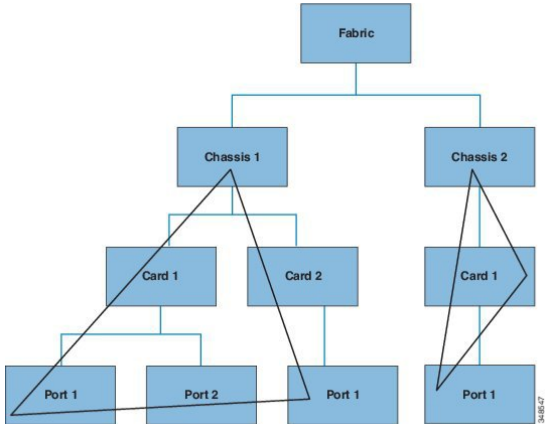
Figure 113: Tree-Level Queries
