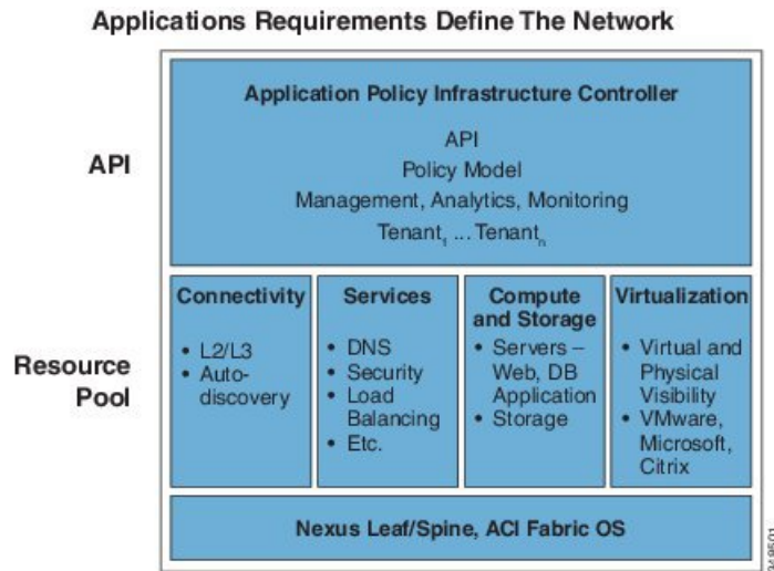
Figure 1: APIC Overview
