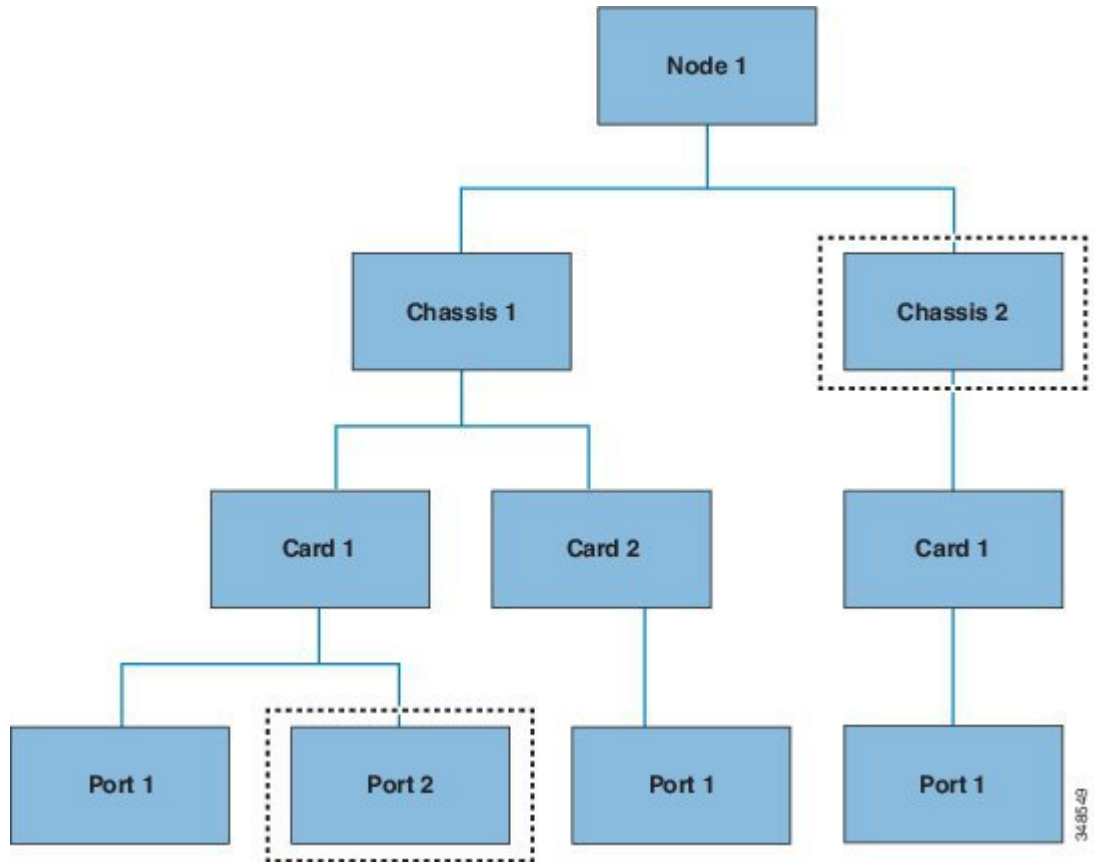
Figure 115: Object-Level Queries
