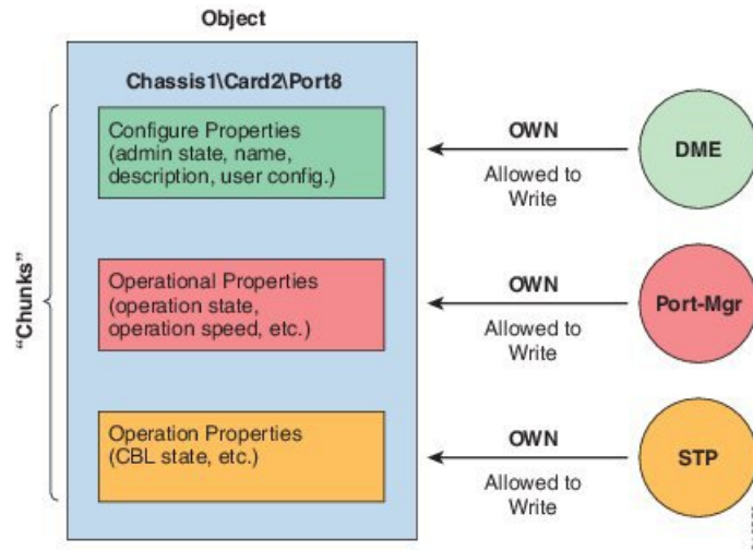
Figure 116: Managed Object Properties
