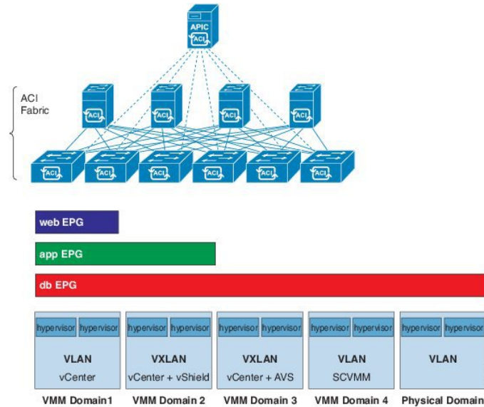
Figure 94: Multiple VMM Domains and Scaling of EPGs in the Fabric
