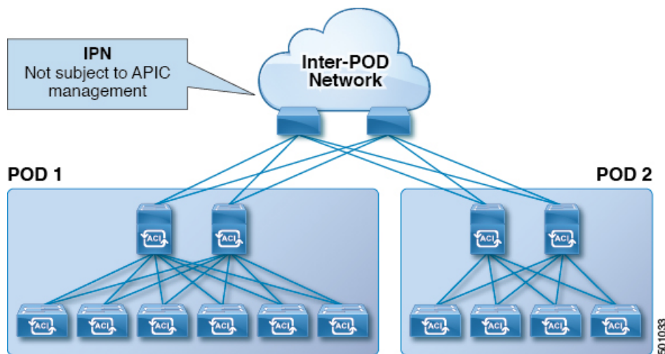
Figure 82: Multi-Pod Topology
