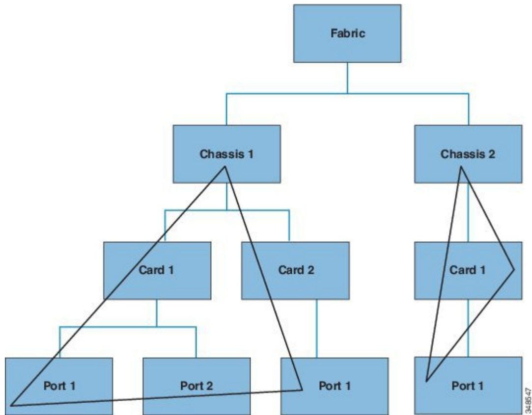
Figure 117: Tree-Level Queries
