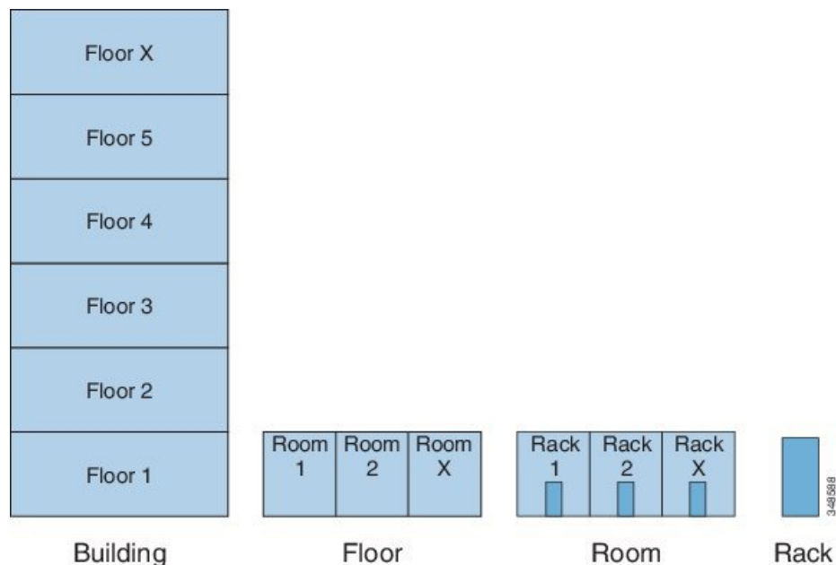
Figure 37: Geolocation
