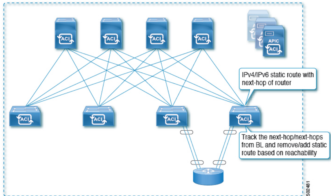
Figure 48: Static Route Availability by Tracking the Next-Hop
