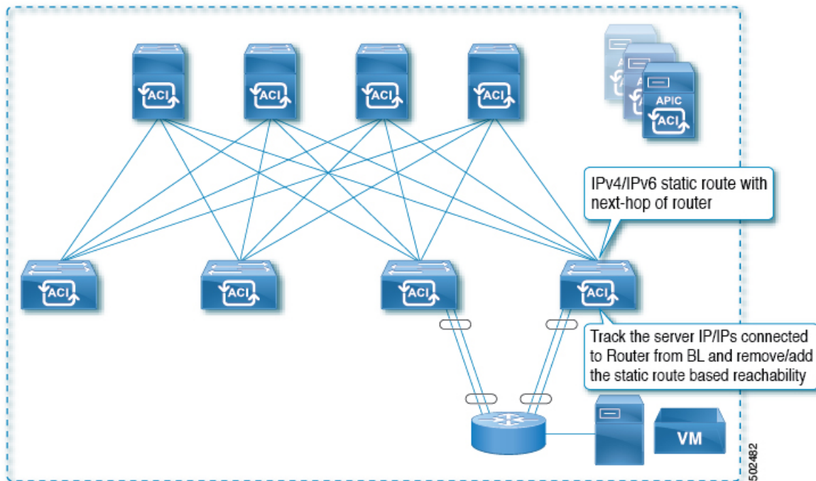
Figure 49: Static Route Availability by Tracking an IP Address Through L3Out
