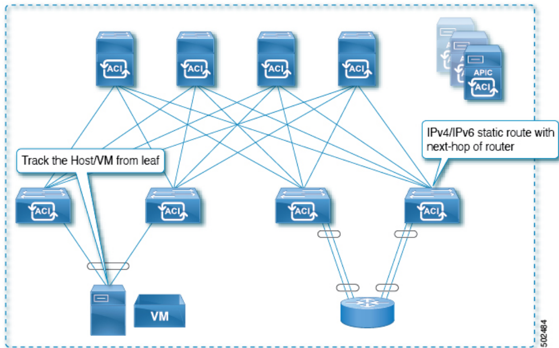
Figure 51: Static Route Availability by Tracking an IP Address in the ACI Fabric
