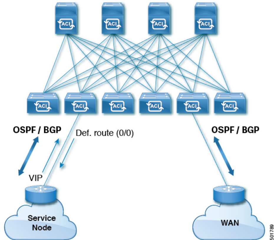
Figure 42: Service Node Transit Connectivity
