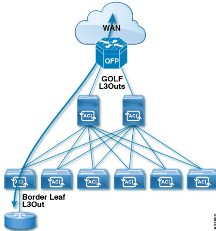
Figure 44: GOLF L3Outs and a Border Leaf L3Out in a Transit-Routed Configuration
