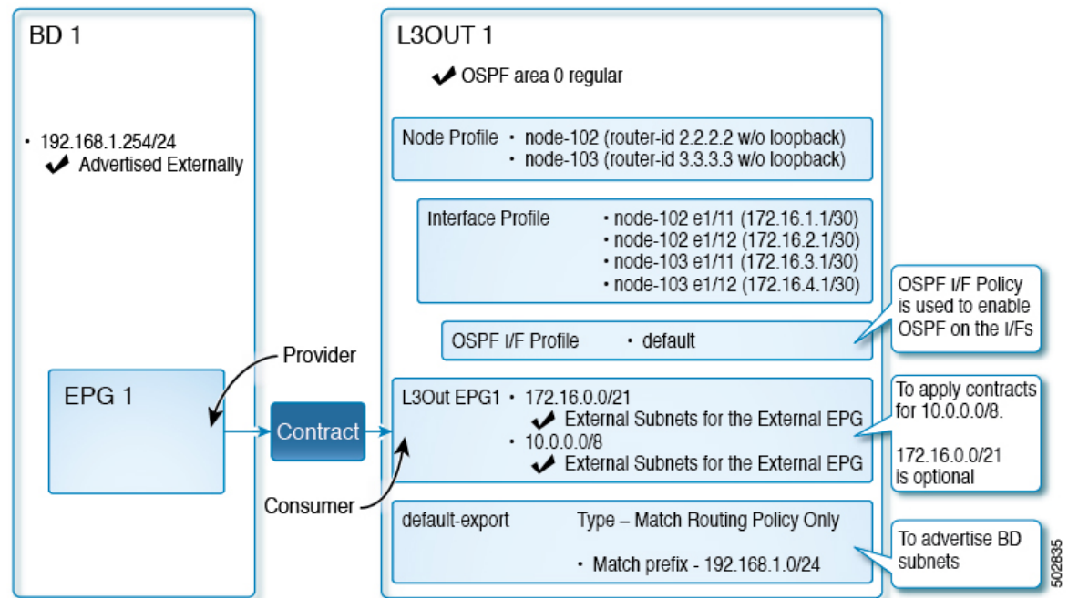
Figure 30: OSPF Configuration Diagram
