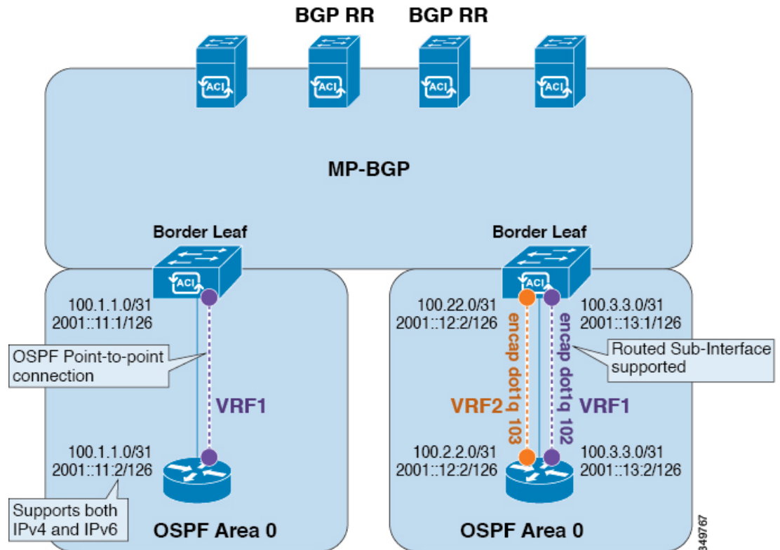
Figure 37: OSPF Layer3 Out Connections
