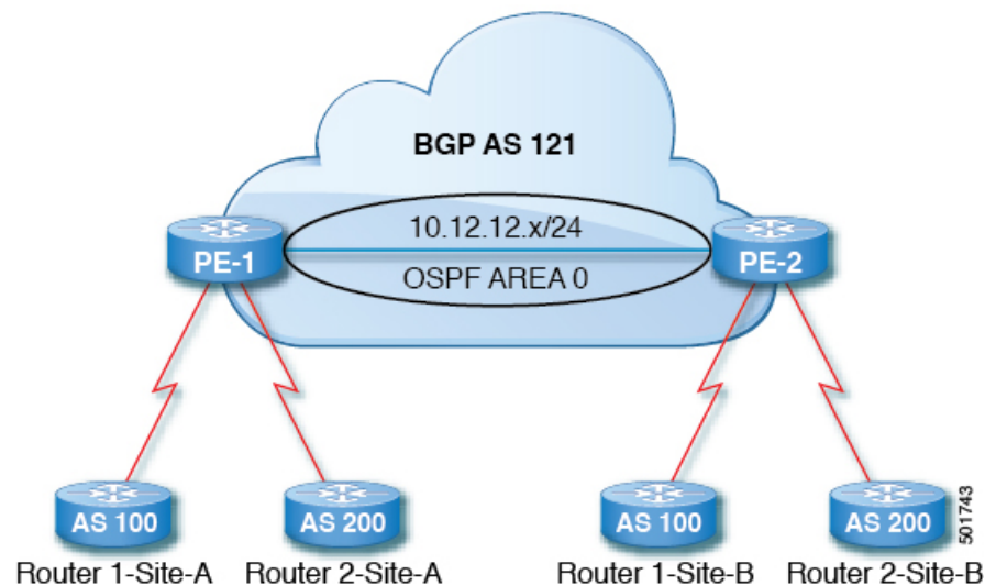
Figure 35: Example Topology Illustrating the Autonomous System Override Process
