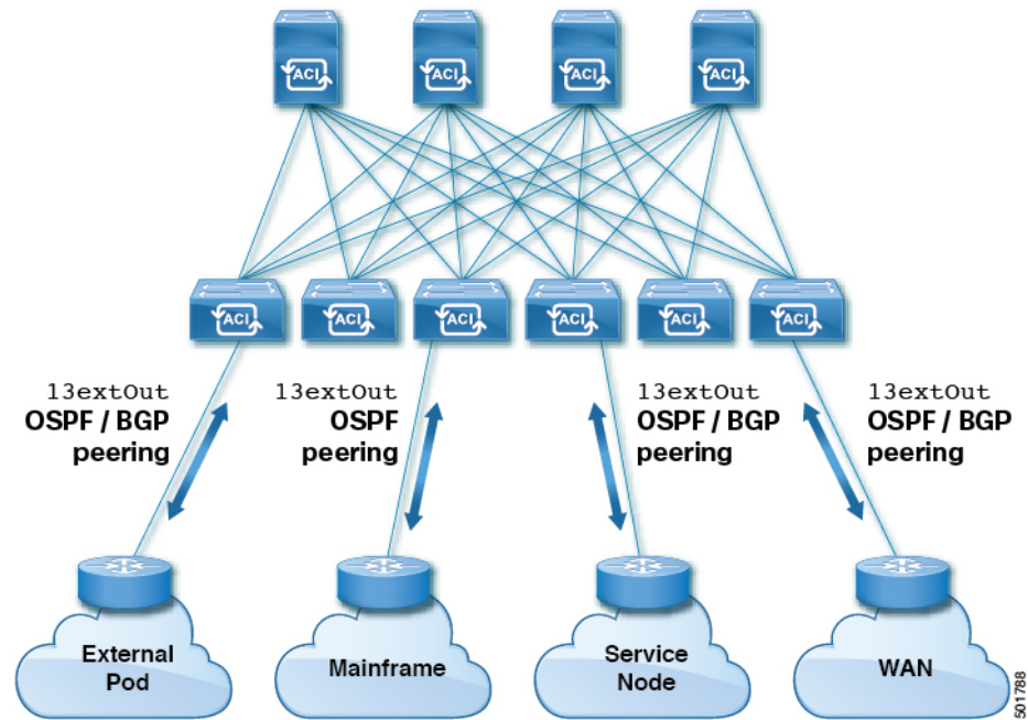
Figure 40: Transit Routing Between Layer 3 Domains
