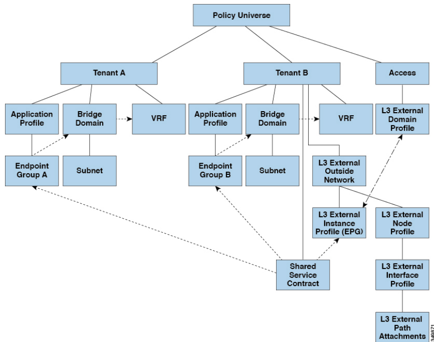
Figure 46: Shared L3Out Policy Model
