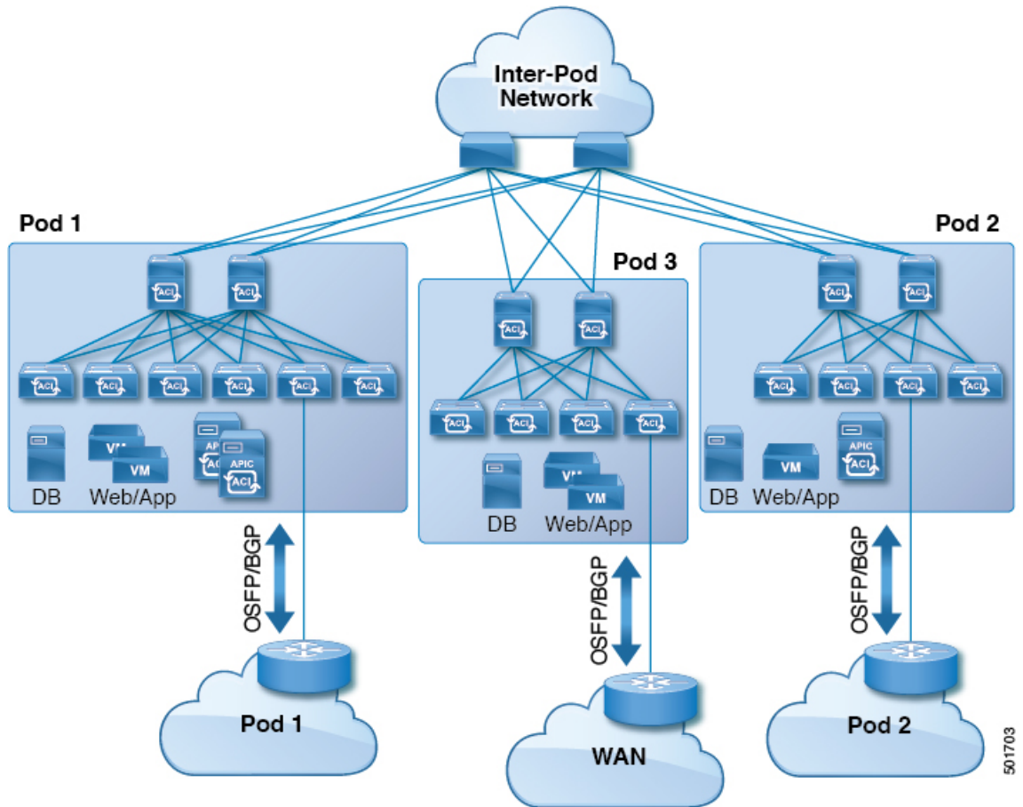
Figure 43: Multiple Pods with L3Outs in a Transit-Routed Configuration
