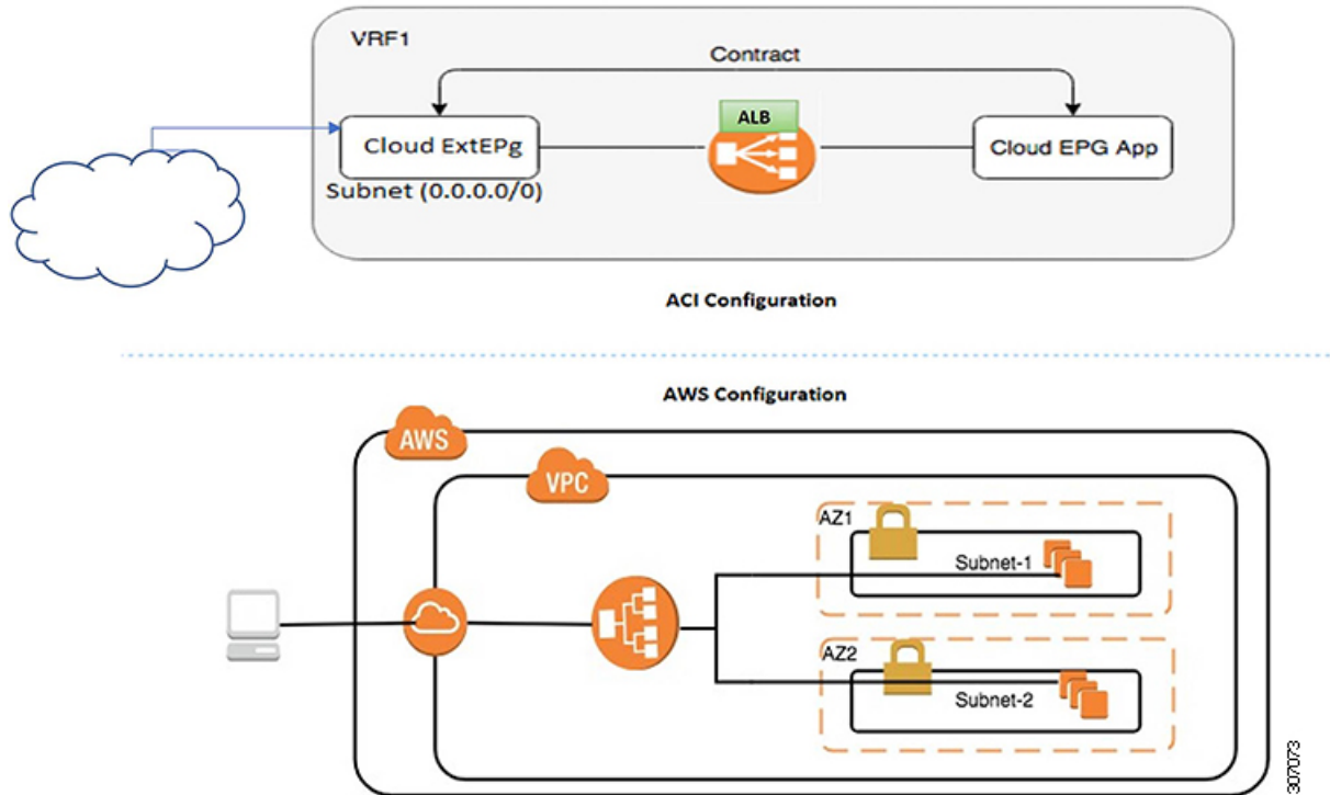
Figure 19: Internet-Facing Deployment
