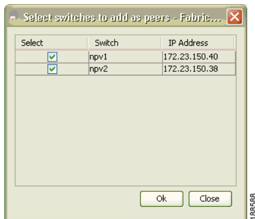
Figure 13-7 Peer Selection
