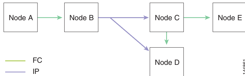
Figure 13-3 Network Example 2 with Fibre Channel and IP Connections
